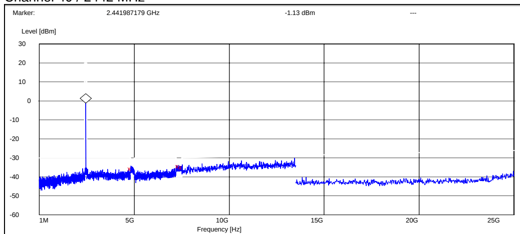
Channel 40 / 2442 MHz
