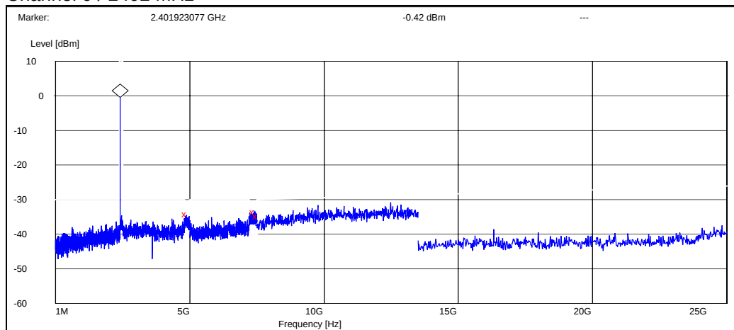
Channel 0 / 2402 MHz
