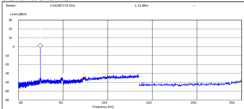
Channel 40 / 2442 MHz
