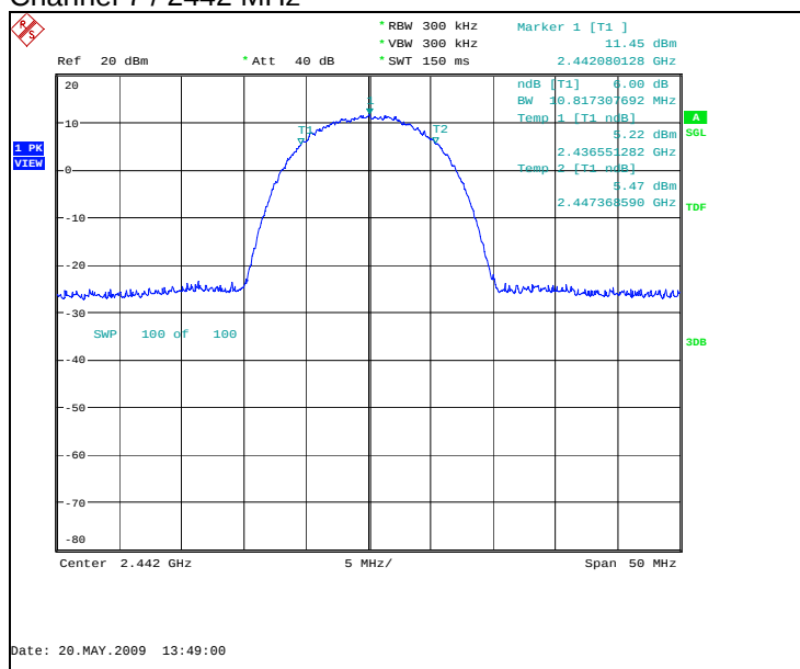
Channel 7 / 2442 MHz
