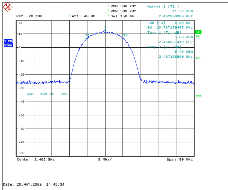
Channel 11 / 2462 MHz
