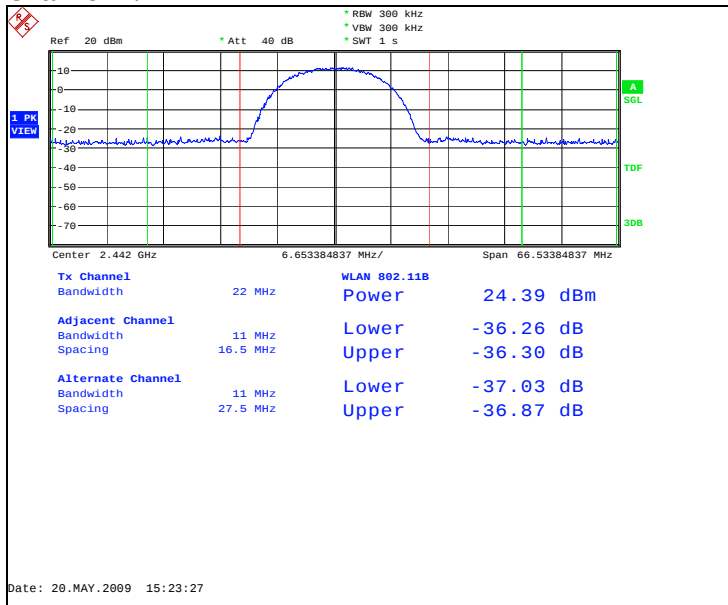
Channel 7 / 2442 MHz
