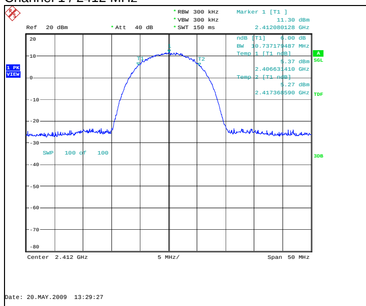
Channel 1 / 2412 MHz
