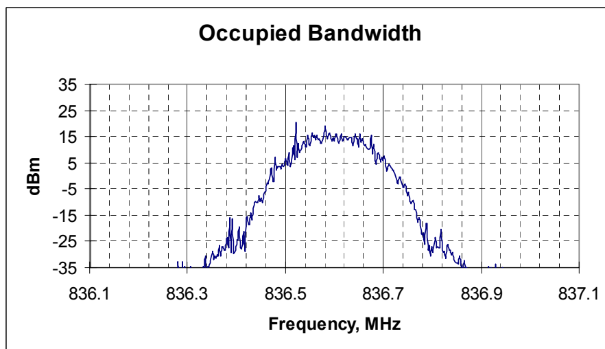
Picture 5. 99% occupied bandwidth, EGPRS channel 190 RBw = VBw = 3KHz, Channel spacing = 200KHz
