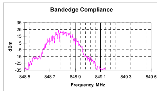
Picture 7. Upper bandedge, channel 251 GSM RBw 3KHz VBw 3KHz
