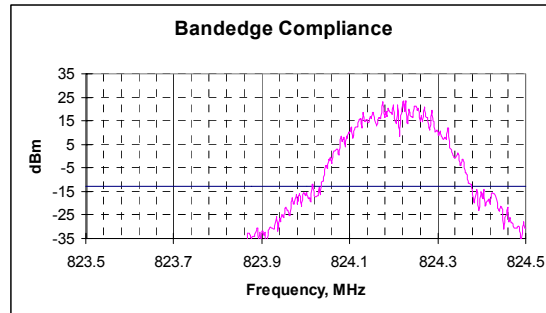
Picture 6. Lower bandedge, channel 128 GSM RBw 3KHz, VBw 3KHz
