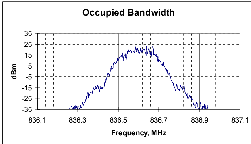
Picture 4. 99% occupied bandwidth, GSM channel 190 RBw = VBw = 3KHz, Channel spacing = 200KHz
