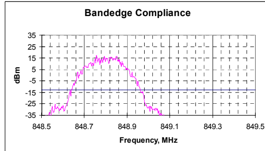
Picture 9. Upper bandedge, channel 251 EGPRS RBw 3KHz VBw 3KHz
