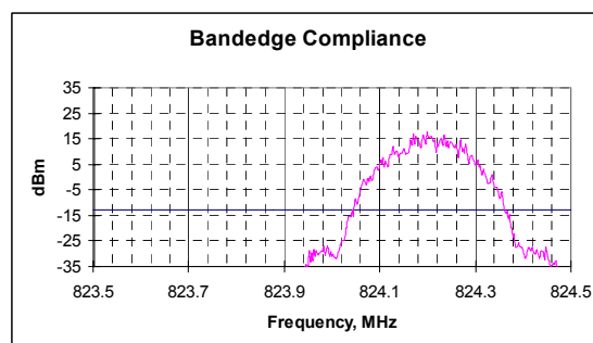
Picture 8. Lower bandedge, channel 128 EGPRS RBw 3KHz VBw 3KHz
