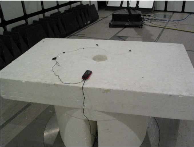
Picture 3 Radiated emission measurement GSM RX + GPS receiver on / FM radio on
