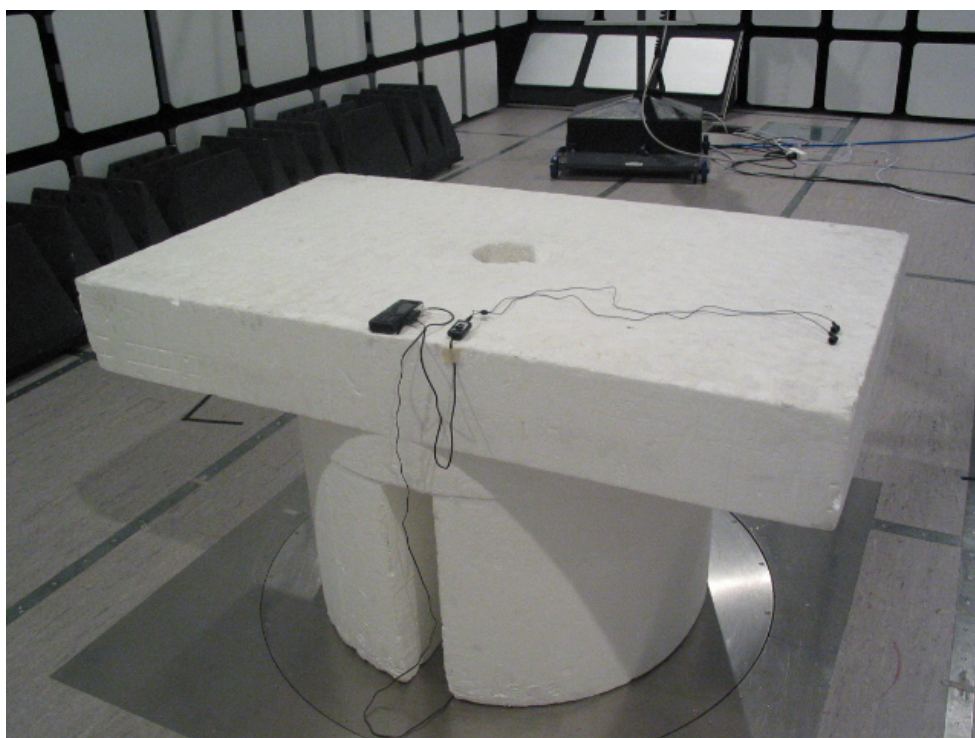
Picture 2 Radiated emission measurement (GSM 1900+FM radio)
