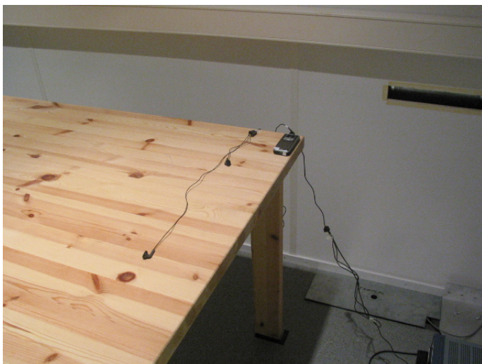
Picture 3 AC powerline conducted emission measurement Bluetooth TX
