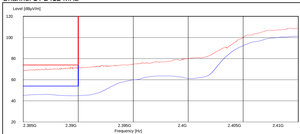
Channel 1 / 2412 MHz
