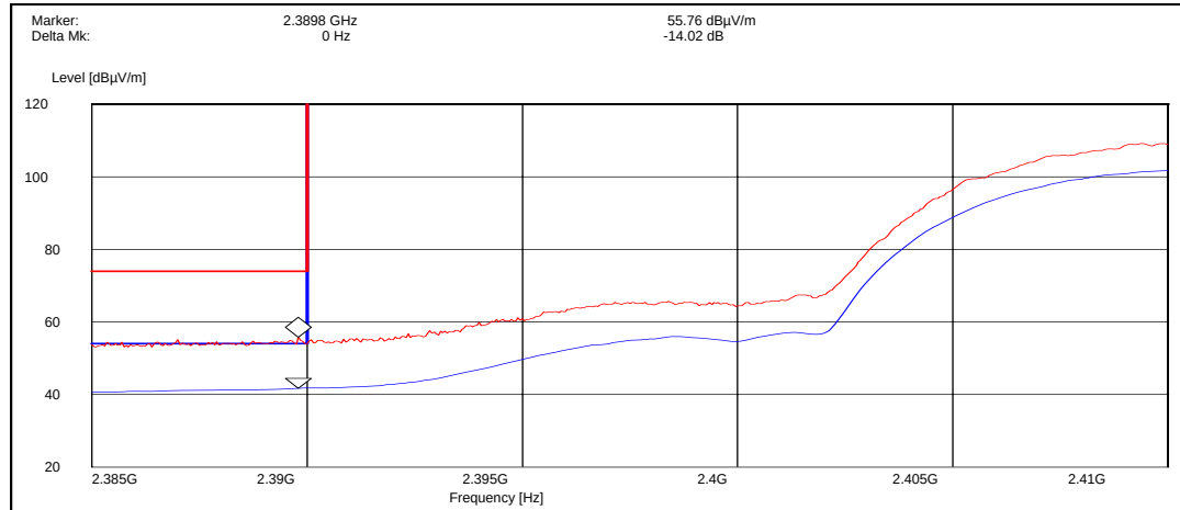
Channel 1 / 2412 MHz
