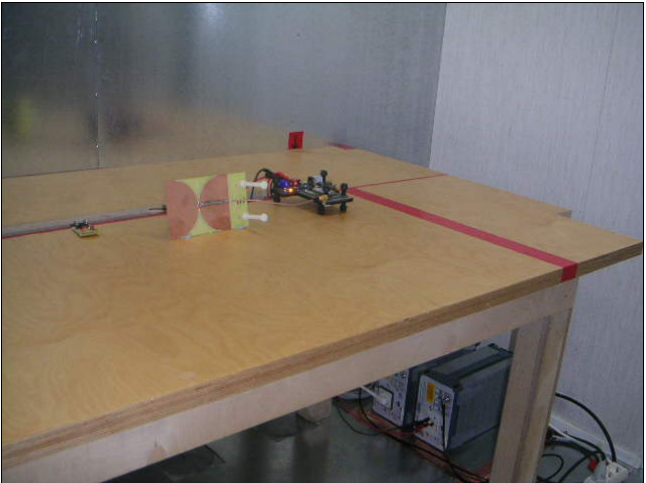
Picture 3 AC powerline conducted emission measurement GSM RX/GPRS, EDGE and WCDMA
