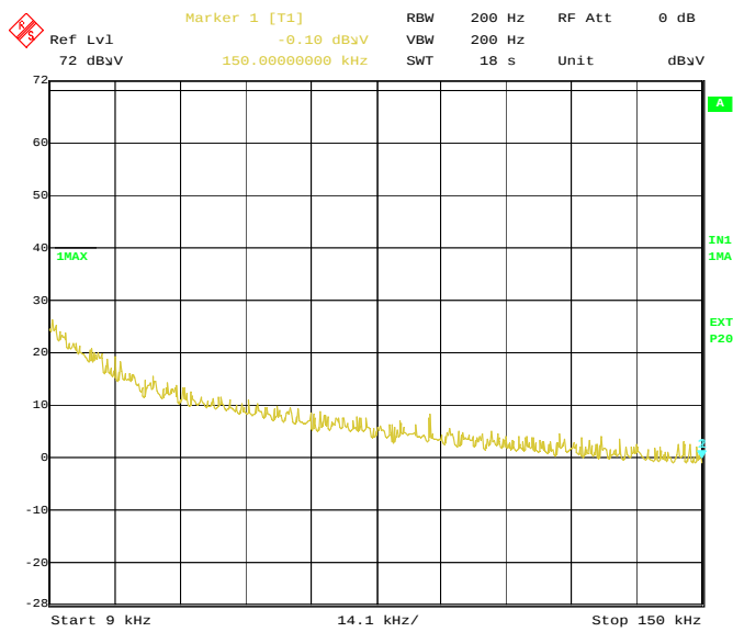
Date: 7.APR.2006 08:31:08 Radiated Emission 9 – 150 kHz
