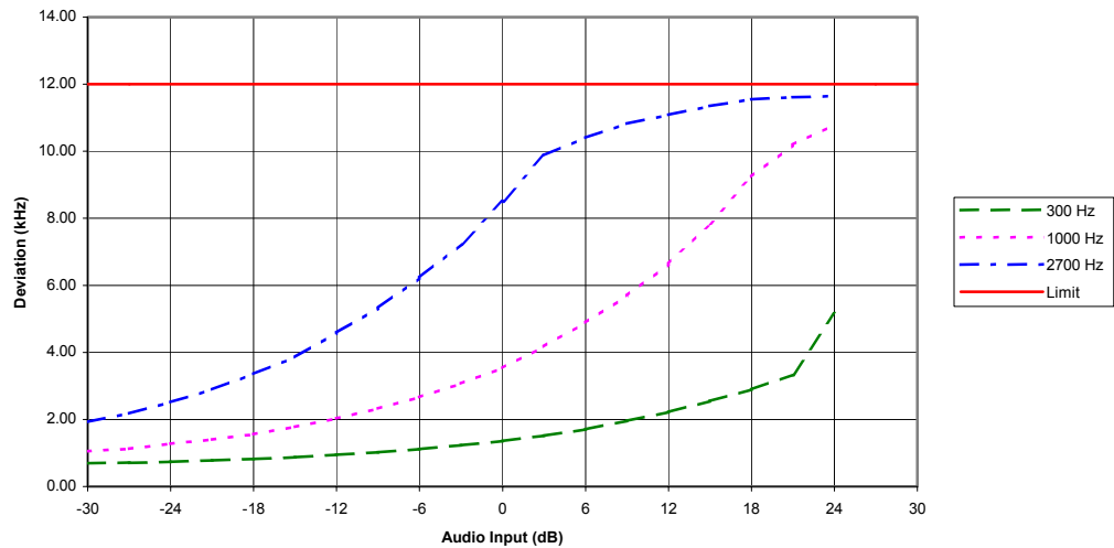
Modulation Limiting - Voice Only, Negative Peaks
