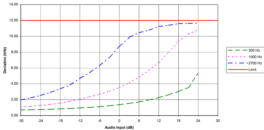
Modulation Limiting - Voice Only, Positive Peaks
