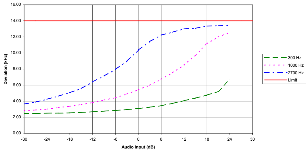
Modulation Limiting - Voice+SAT, Negative Peaks
