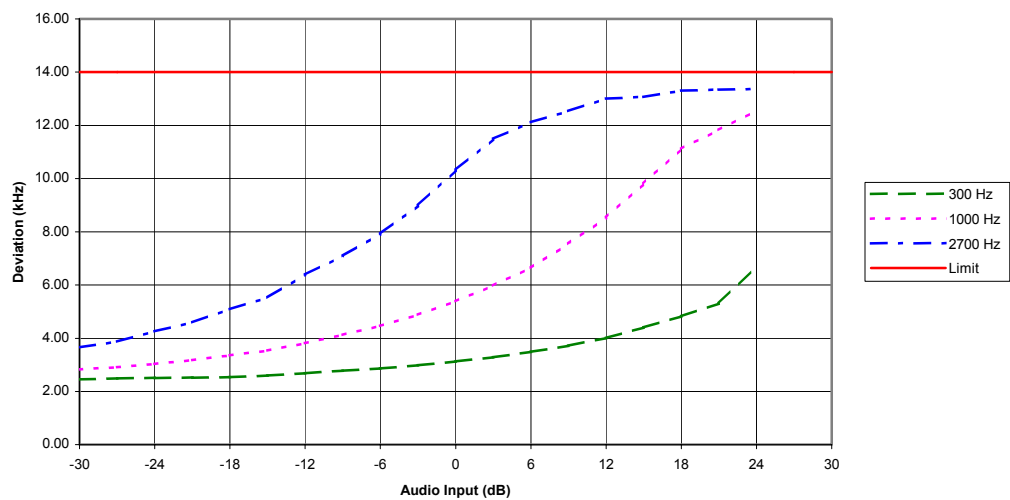
Modulation Limiting - Voice+SAT, Positive Peaks
