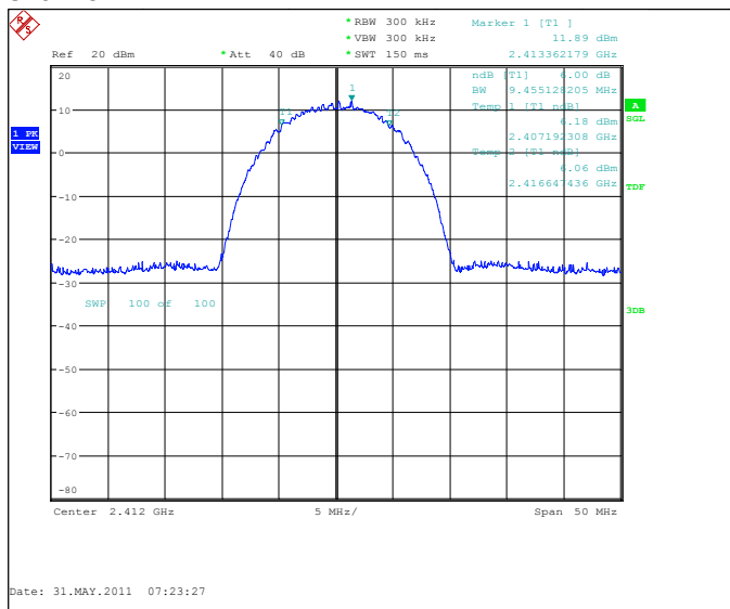
Channel 1 / 2412 MHz
