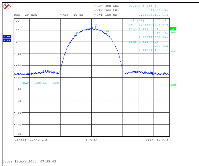
Channel 7 / 2442 MHz
