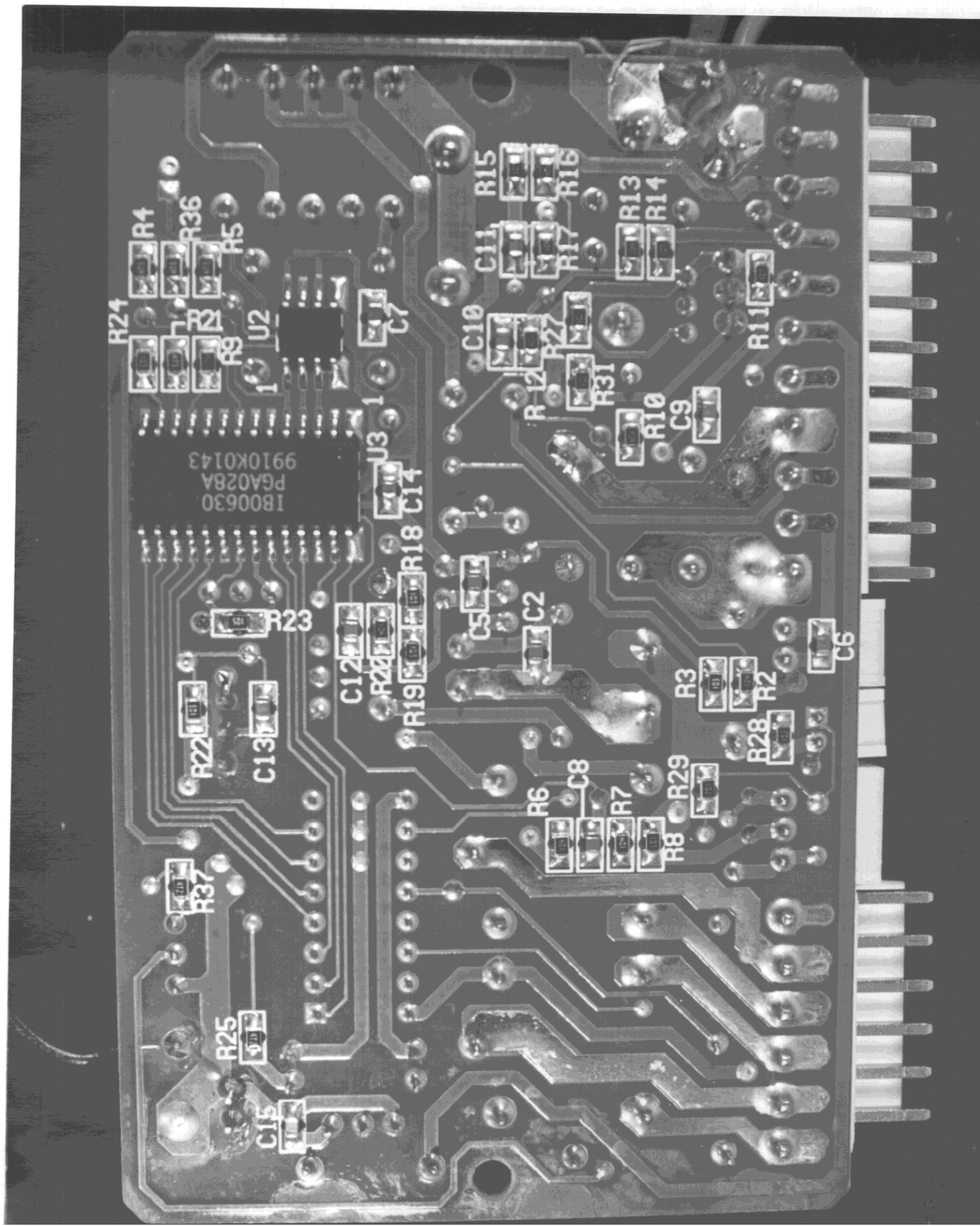
Solder View of PCB
