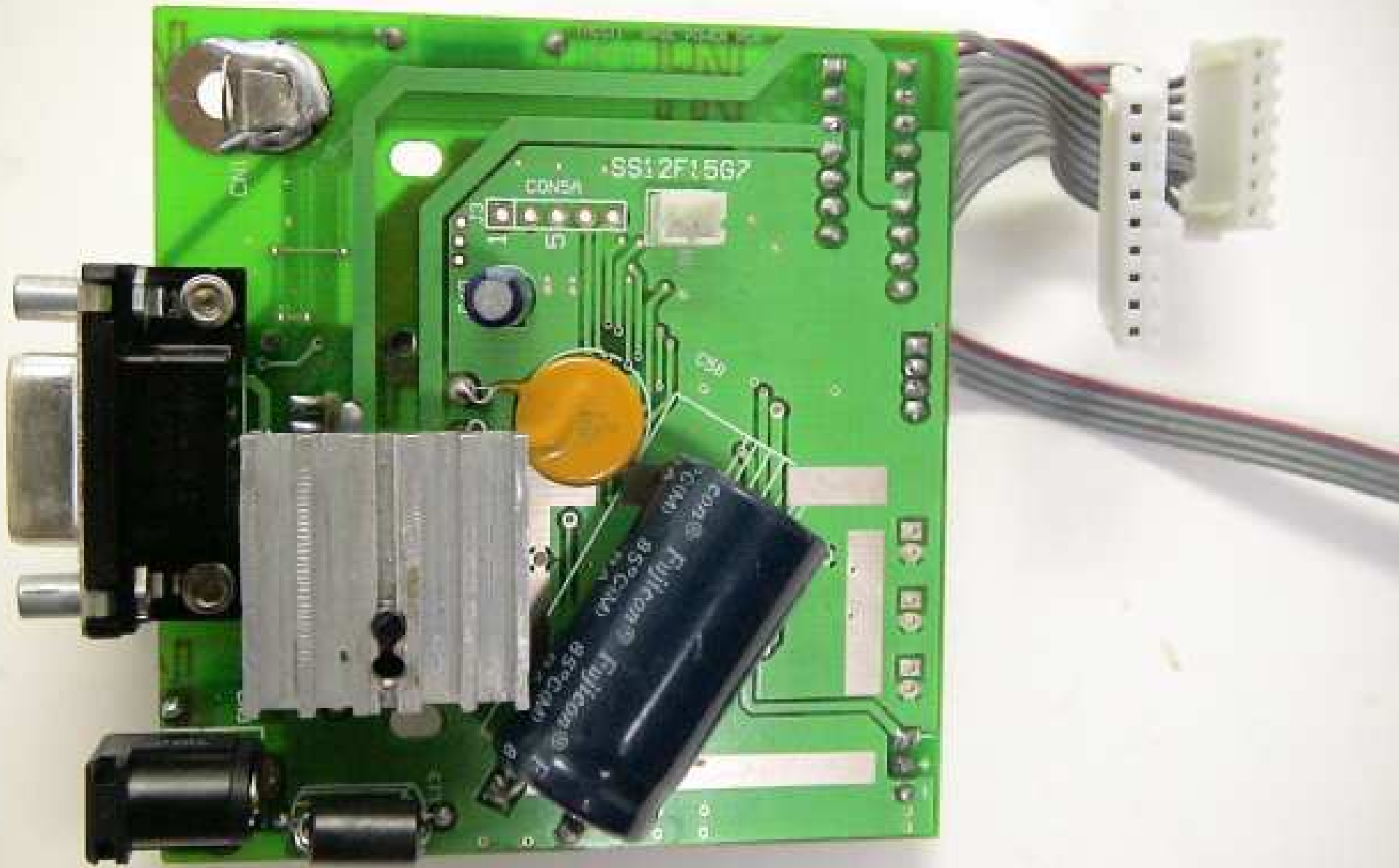
PCB (bottom)
