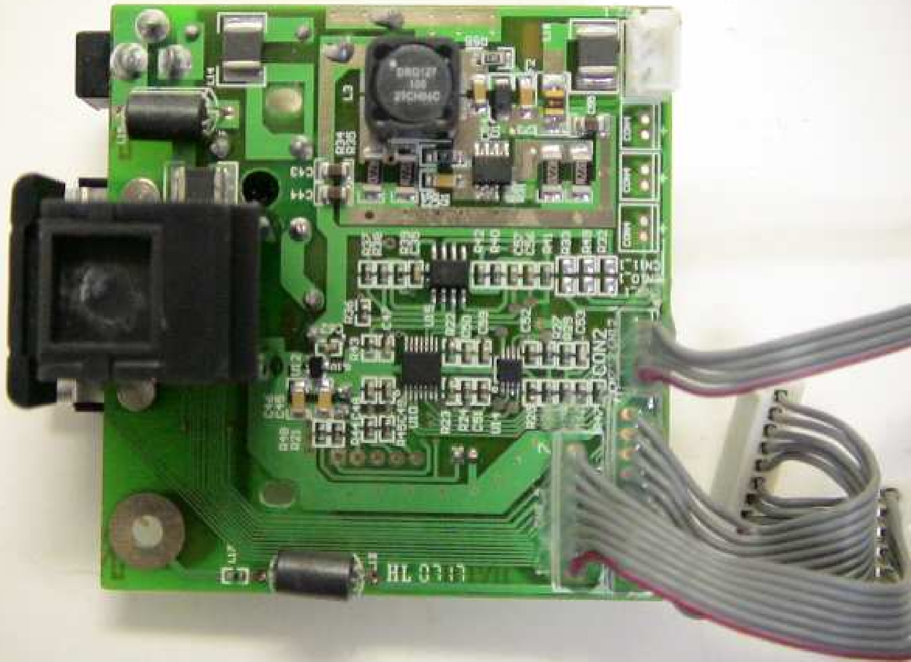
PCB (top)
