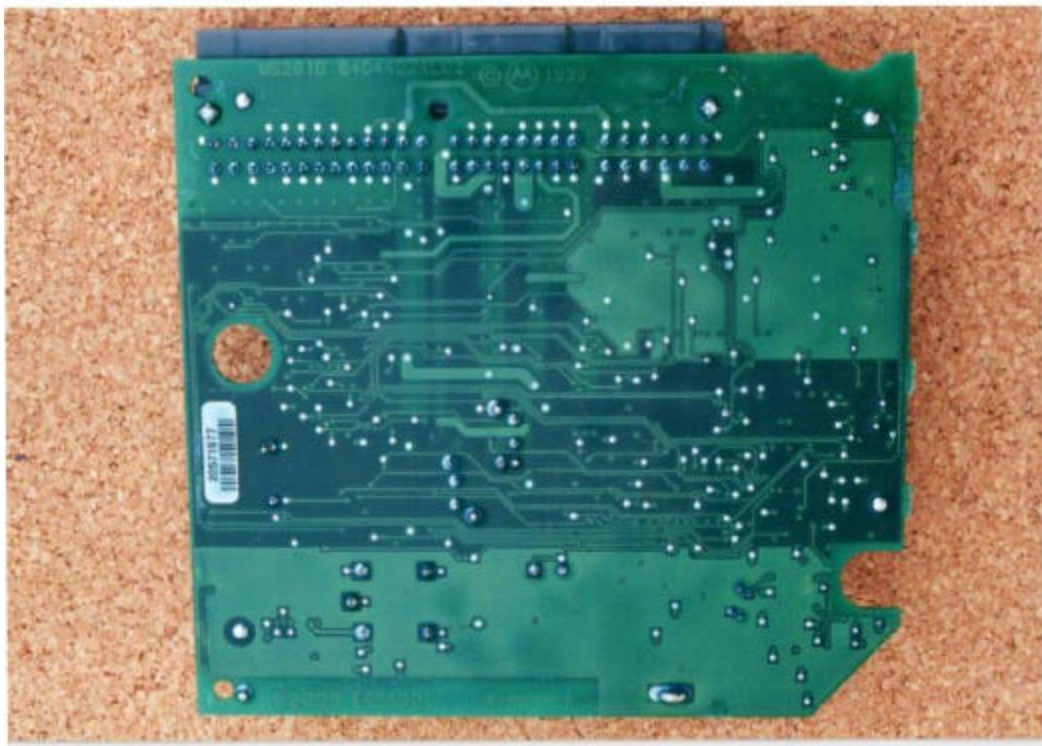
LHJ010 Receiver- PCB Bottom
