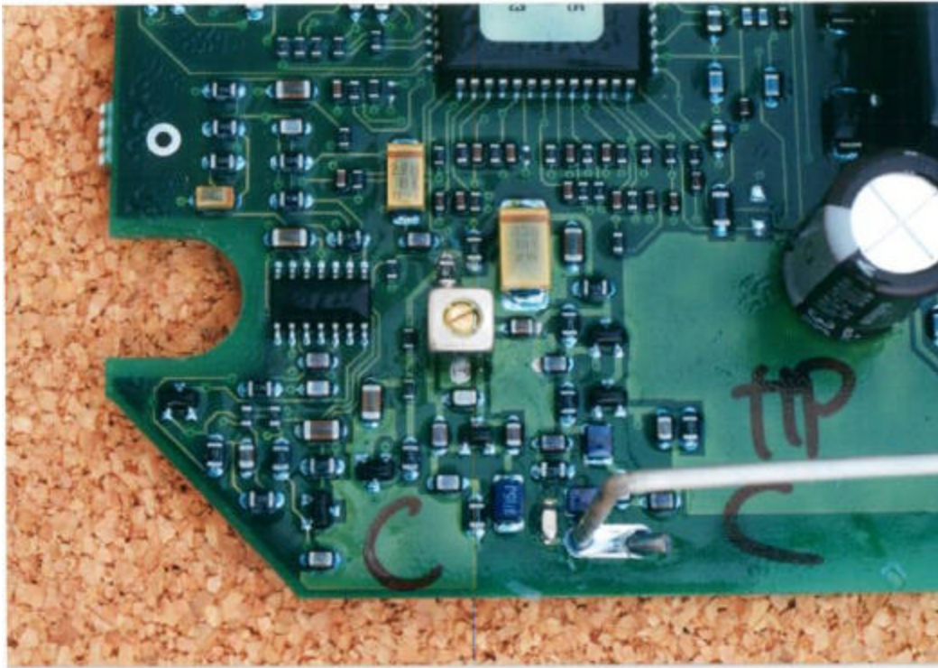
LHJ010 Receiver – PCB RF Top
