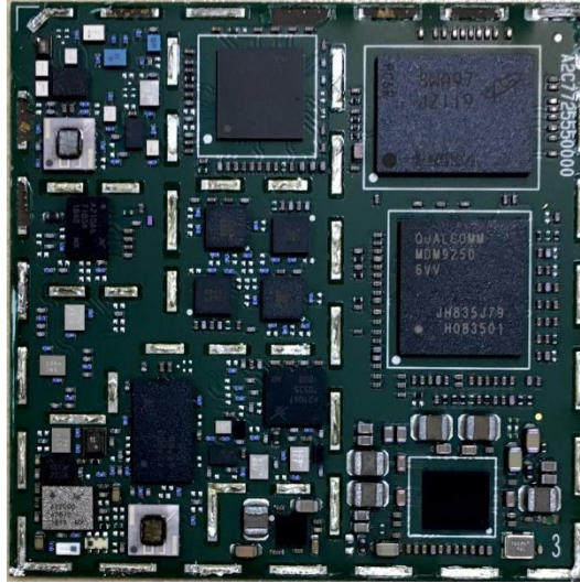
Fig. 3. WT50RW02 module top view with the shield and shield frame removed.
