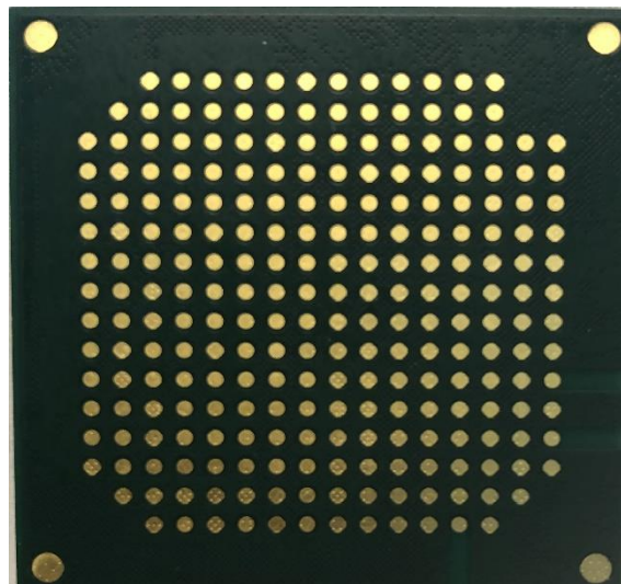
Fig. 4. WT50RW02 module bottom view
