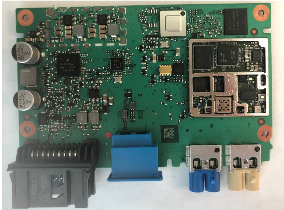
Fig. 5. HNA10_00 bottom view of the pcb with shields removed.
