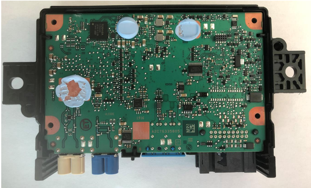
Fig. 3 HNA10_00 device with metal cover removed. Top view on the pcb.
