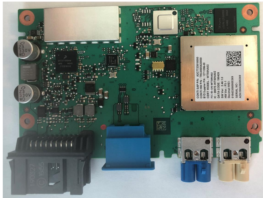
Fig. 4. HNA10_00 bottom view of the pcb with shields.
