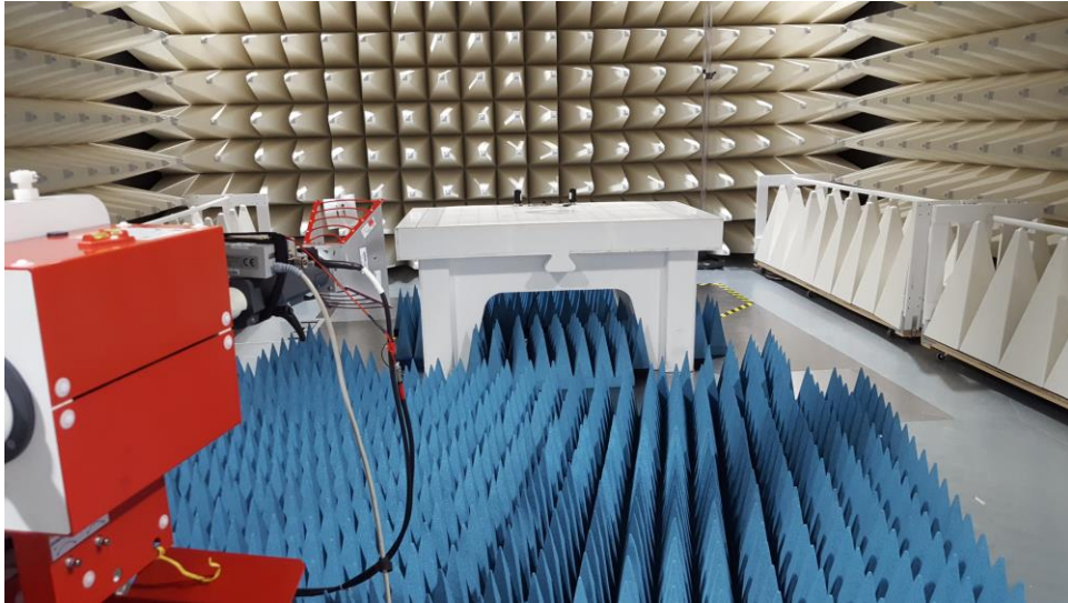
Figure B5. High range Radiated emission Set up Horn antenna
