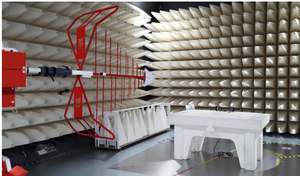
Figure B4. Low range Radiated emission Set up Biconical log antenna
