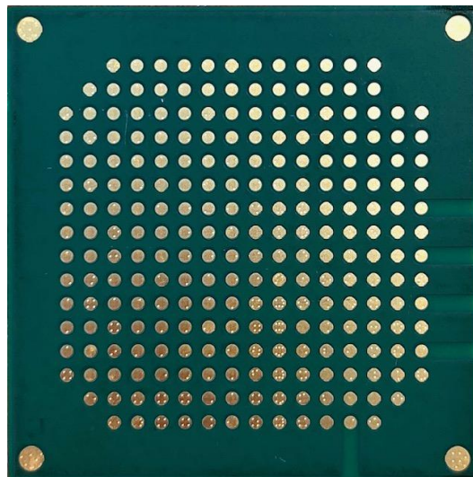
Fig. 4. WT50NA01 module bottom view
