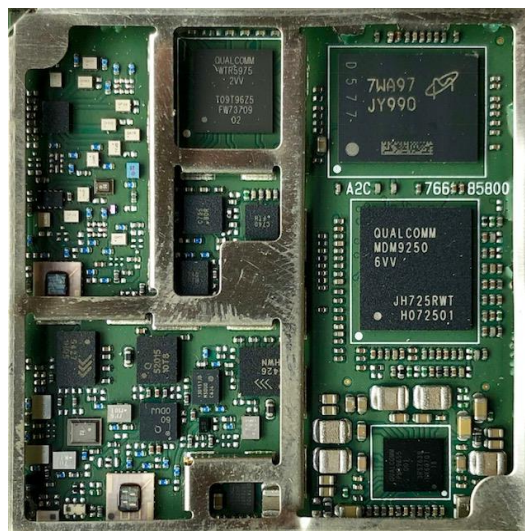
Fig. 2. WT50NA1 top view with the shield removed.
