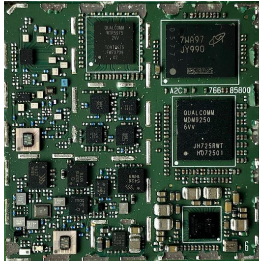
Fig. 3. WT50NA01 module top view with the shield and shield frame removed.
