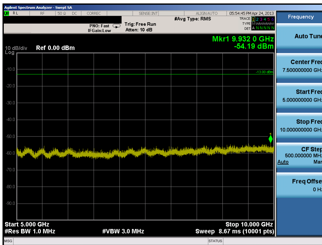
Plot 7-12. Conducted Spurious Plot (10.0MHz QPSK – RB Size 1, RB Offset 0 – Mid Channel)
