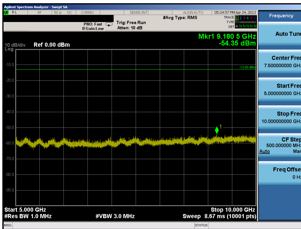
Plot 8-12. Conducted Spurious Plot (10.0MHz QPSK – RB Size 1, RB Offset 0 – Low Channel)
