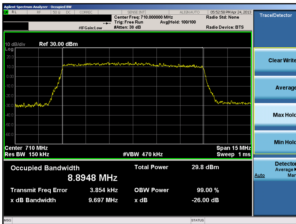
Plot 7-8. Occupied Bandwidth Plot (10.0MHz 16-QAM – RB Size 50)
