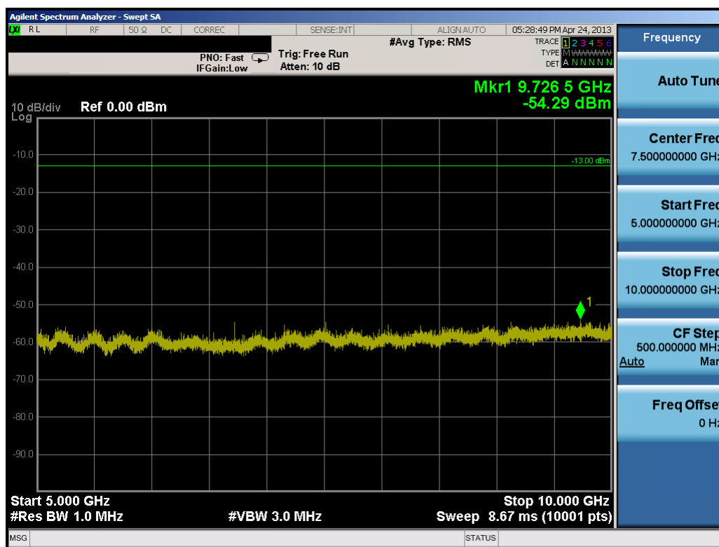
Plot 8-16. Conducted Spurious Plot (10.0MHz QPSK – RB Size 1, RB Offset 0 – High Channel)
