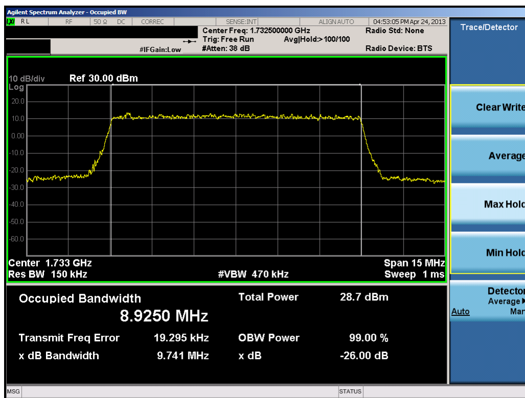
Plot 9-12. Occupied Bandwidth Plot (10.0MHz 16-QAM – RB Size 50)
