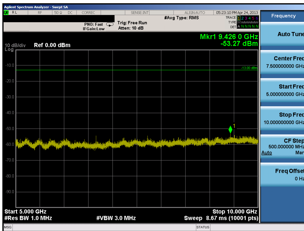
Plot 8-14. Conducted Spurious Plot (10.0MHz QPSK – RB Size 1, RB Offset 0 – Mid Channel)
