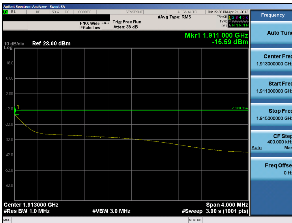
Plot 10-6. Upper Extended Band Edge Plot (5.0MHz QPSK – RB Size 25)
