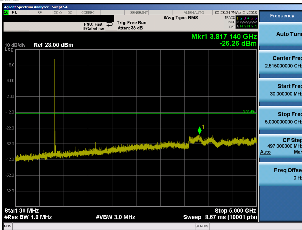
Plot 8-15. Conducted Spurious Plot (10.0MHz QPSK – RB Size 1, RB Offset 0 – High Channel)
