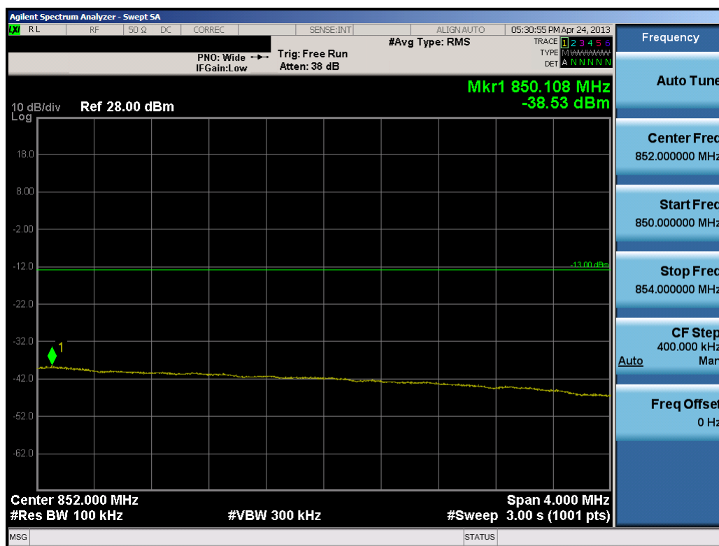
Plot 8-18. Upper Extended Band Edge Plot (10.0MHz QPSK – RB Size 50)
