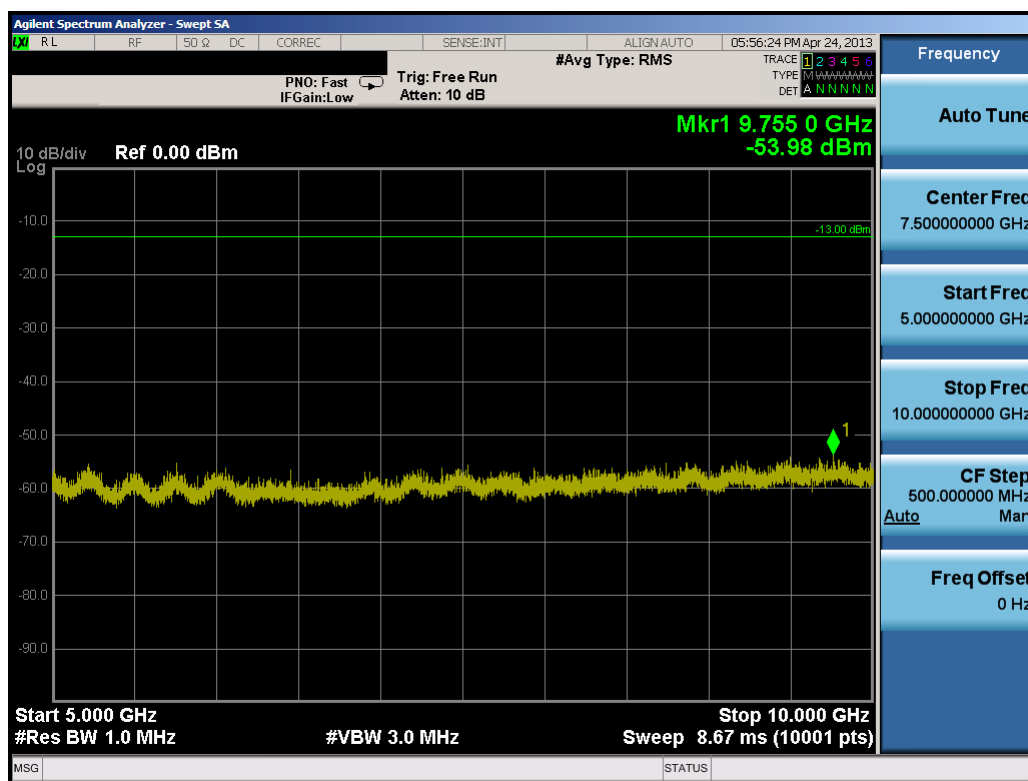
Plot 7-10. Conducted Spurious Plot (10.0MHz QPSK – RB Size 1, RB Offset 0 – Low Channel)
