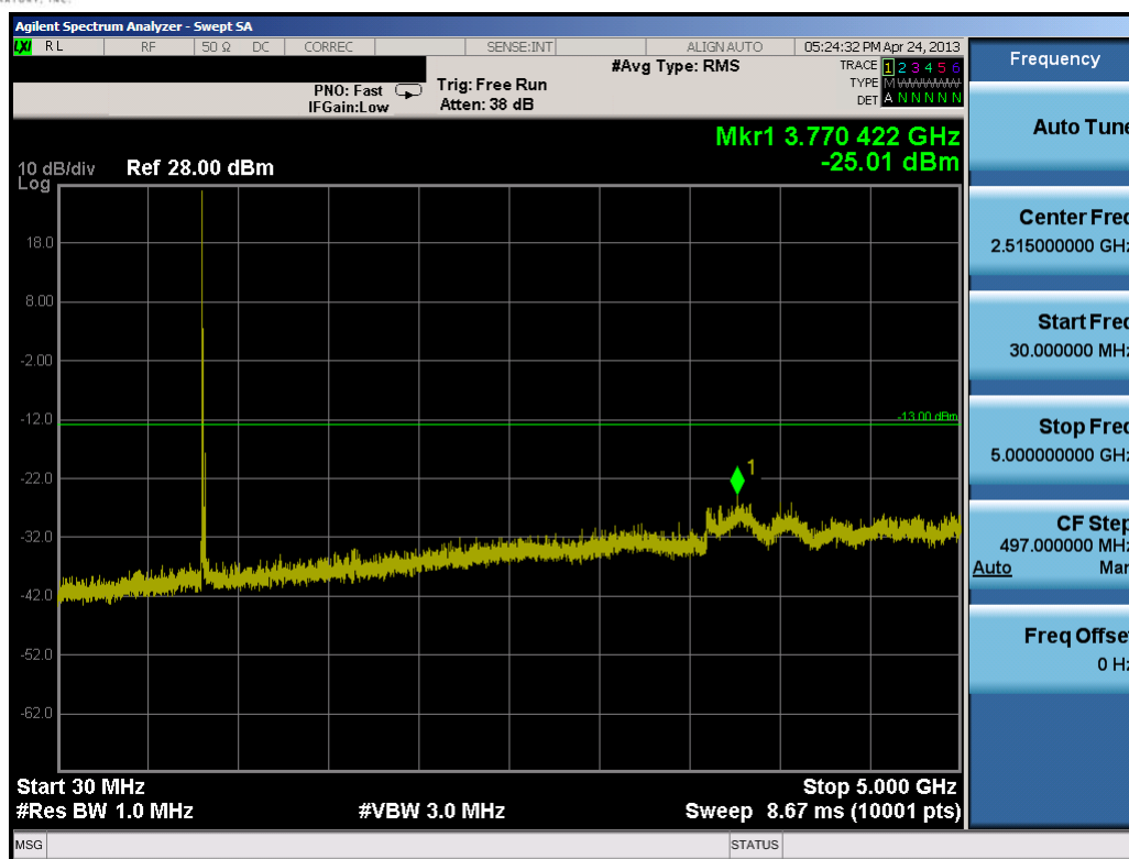
Plot 8-11. Conducted Spurious Plot (10.0MHz QPSK – RB Size 1, RB Offset 0– Low Channel)
