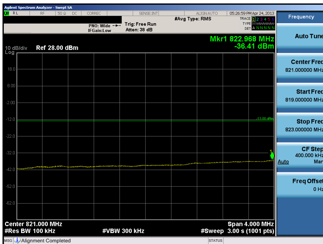
Plot 8-8. Lower Extended Band Edge Plot (10.0MHz QPSK – RB Size 50)
