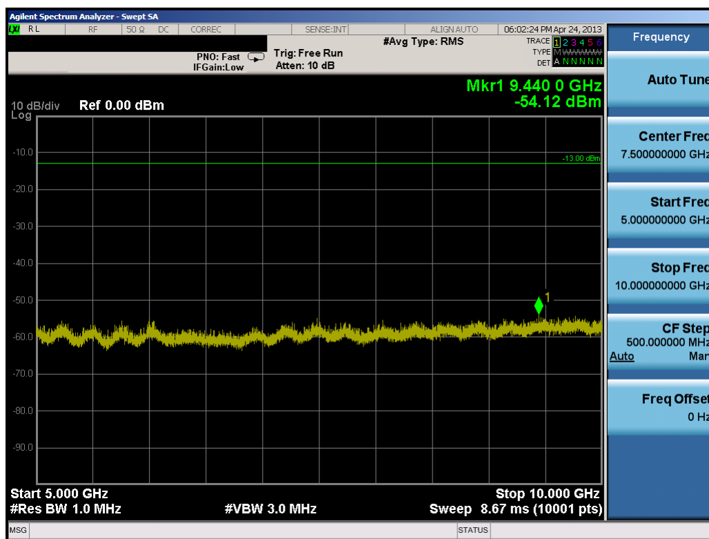
Plot 7-14. Conducted Spurious Plot (10.0MHz QPSK – RB Size 1, RB Offset 0 – High Channel)
