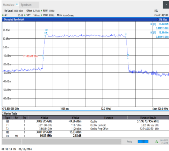
1-N77-3700-3980-30-60-M-3-DFT-16QAM-Outer_Ful I-162@0-Ant2-57.794-60.840-≤60-PASS
