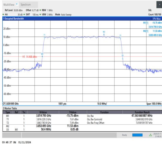
1-N77-3700-3980-30-50-M-9-CP-256QAM-Outter_Fu ll-133@0-Ant2-47.564-50.400≤50-PASS
