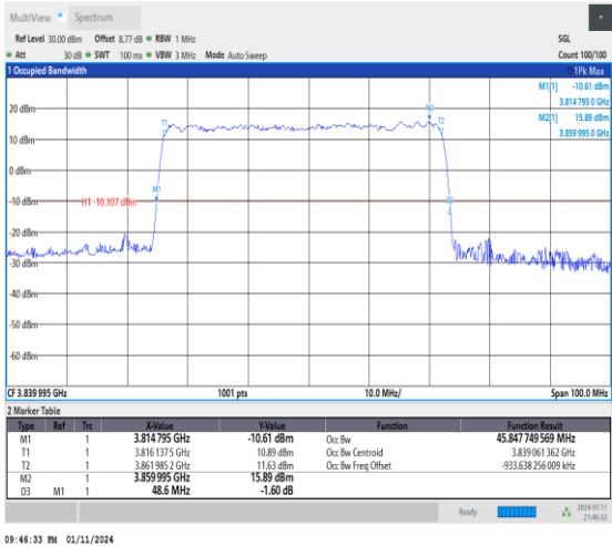
1-N77-3700-3980-30-50-M-3-DFT-16QAM-Out_ull-128@0-Ant2-45.848-48.600-≤50-PASS
