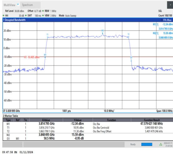
1-N77-3700-3980-30-50-M-7-CP-16QAM-Outter_Full -133@0-Ant2-47.579-50.500≤50-PASS
