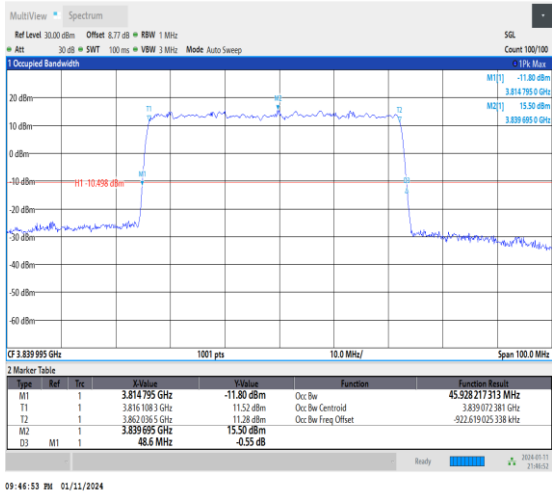
1-N77-3700-3980-30-50-M-4-DFT-64QAM-Out_ull-128@0-Ant2-45.928-48.600-≤50-PASS
