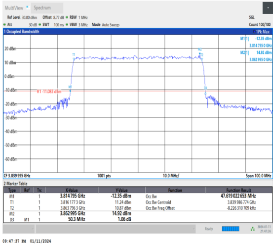
1-N77-3700-3980-30-50-M-6-CP-QPSK-Outter_Full-1 33@0-Ant2-47.619-50.300≤50-PASS
