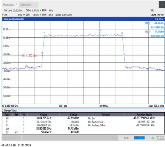
1-N77-3700-3980-30-50-M-8-CP-64QAM-Outter_Full- 133@0-Ant2-47.698-50.400≤50-PASS
