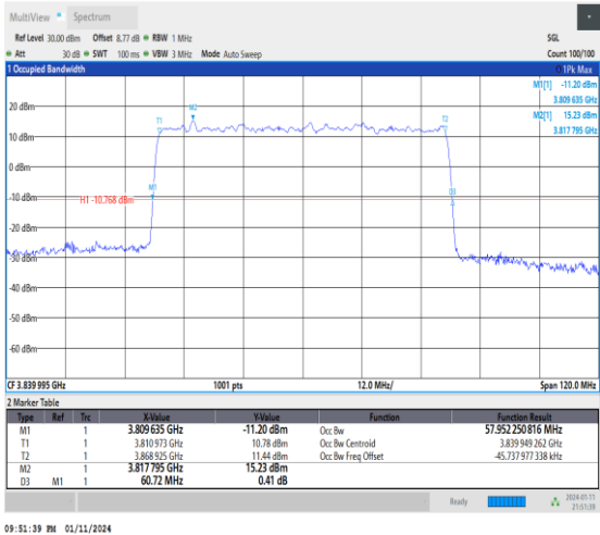
1-N77-3700-3980-30-60-M-4-DFT-64QAM-Outer_Fu ll-162@0-Ant2-57.952-60.720-≤60-PASS
