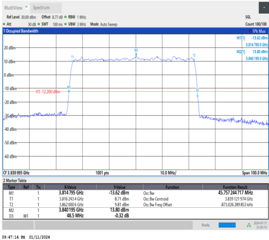
1-N77-3700-3980-30-50-M-5-DFT-256QAM-Out_ull-128@0-Ant2-45.757-48.500-≤50-PASS
