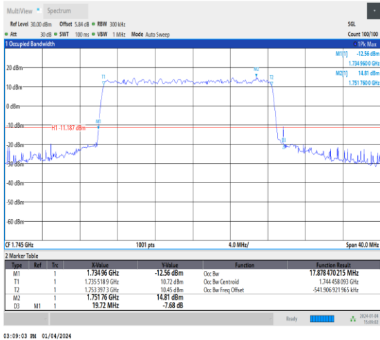
1-N66-15-20-M-1-DFT-QPSK-Outer_Full-100@0-Ant 1-17.878-19.720-≤20-PASS
