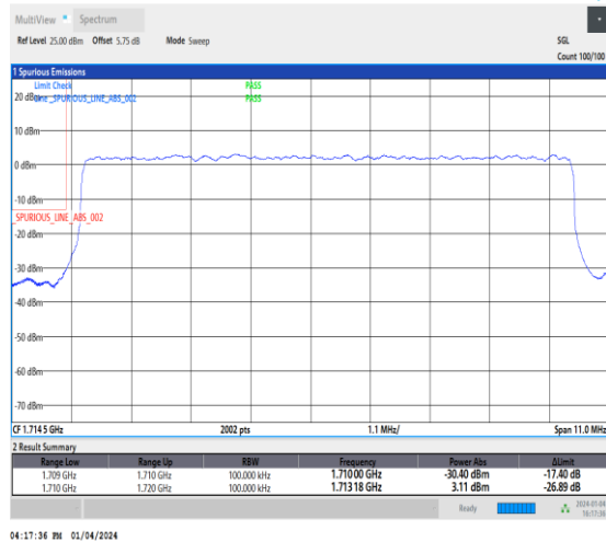
1-N66-15-10-L-3-DFT-PI2BPSK-Outer_Full-50@0-Ant1-1-seegraph-PASS-see graph
