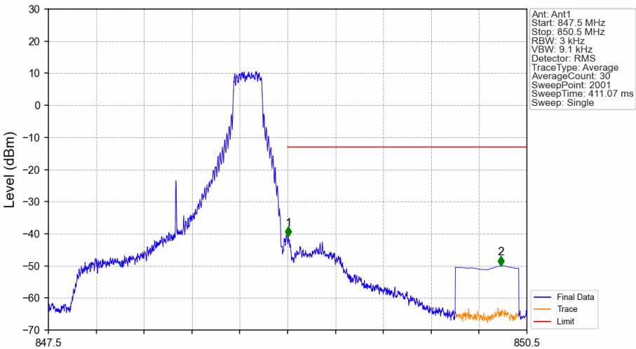
Band26b_1.4MHz_QPSK_HCH_848.3MHz_RB_1_5_NTNV
