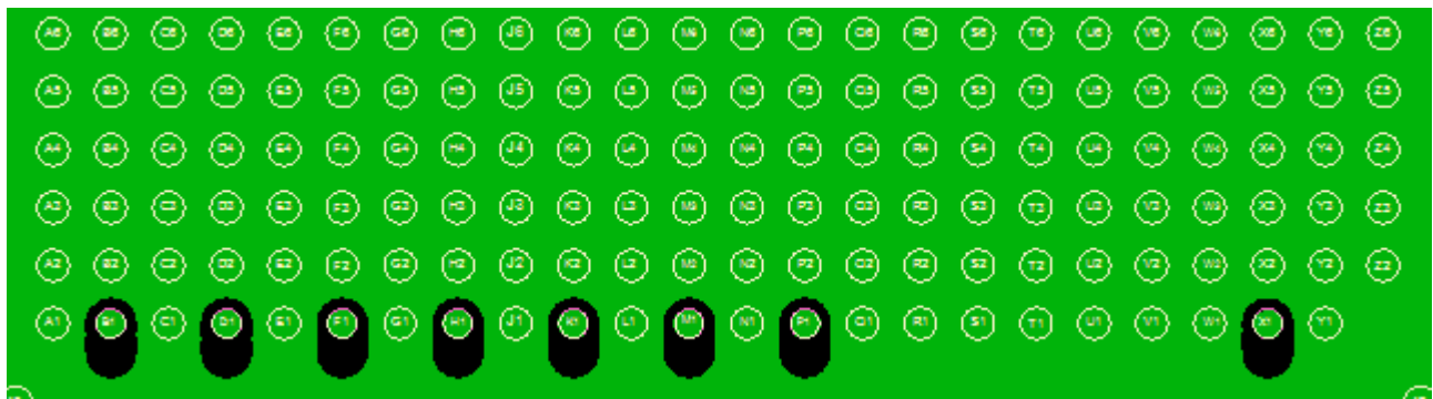
Figure 8-1: Antenna Pad Ground Cutouts (NAD bottom layer)
