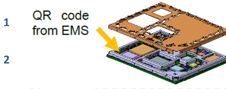
Figure 6-1: Module Exploded View
