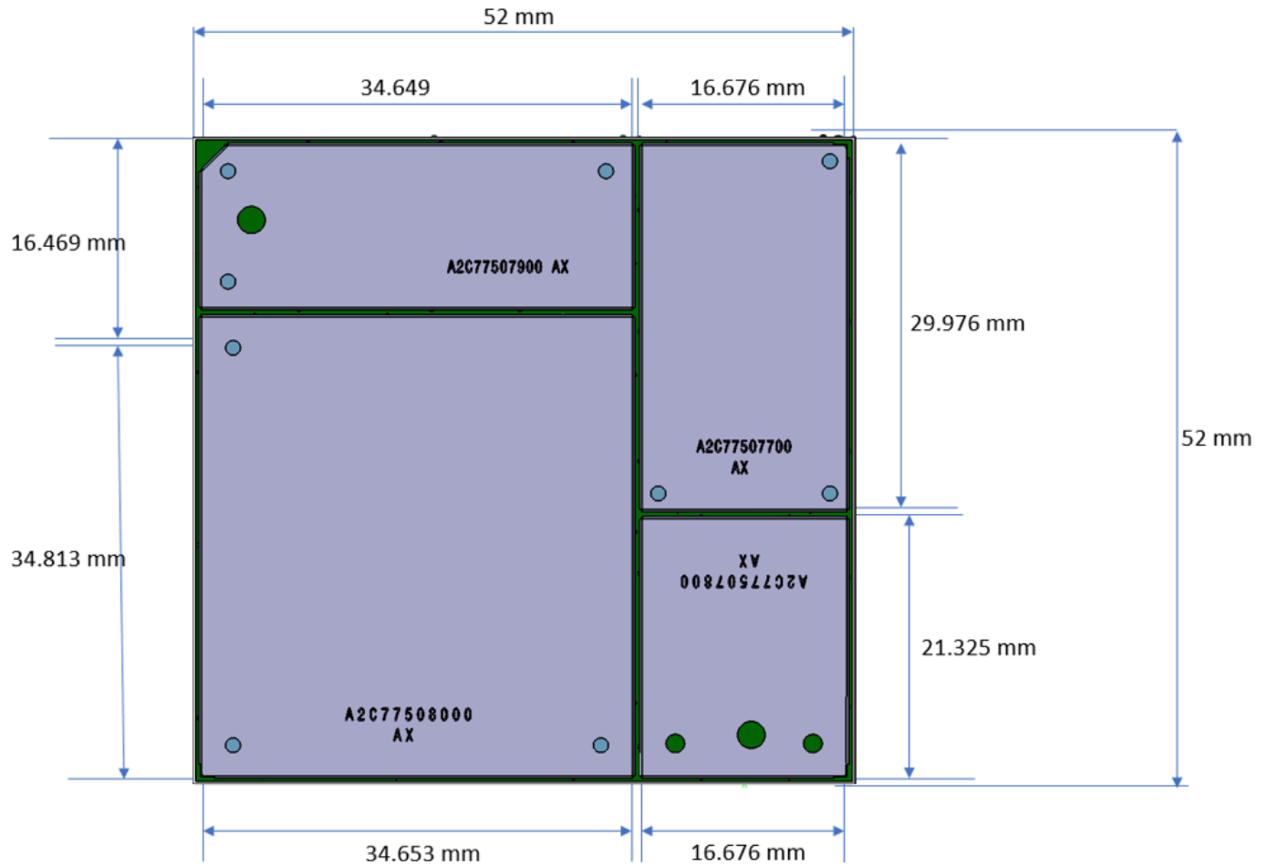
Figure 6-2: Module Top View
