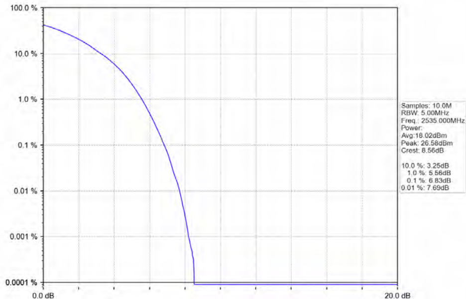
Band7_15MHz_64QAM_MCH_2535MHz_RB_75_0_NTNV
