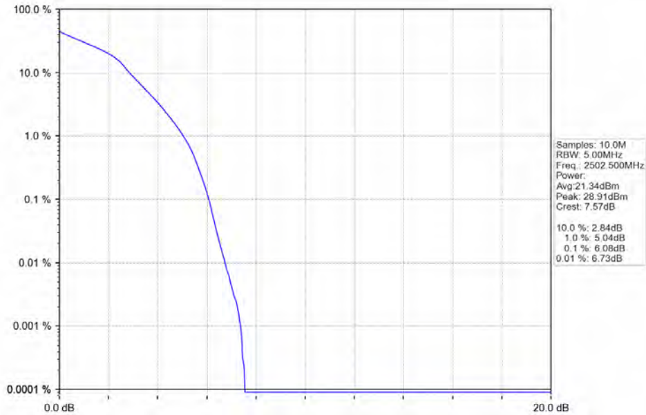
Band7_5MHz_64QAM_LCH_2502.5MHz_RB_25_0_NTNV
