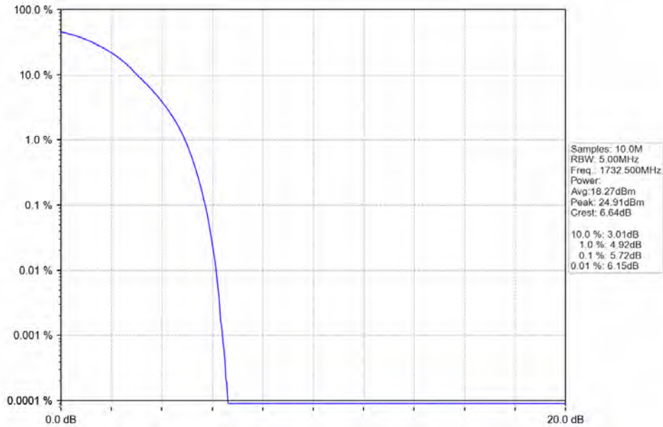
Band 4 15MHz QPSK MCH 1732.5MHz RB 75 0 NTN
