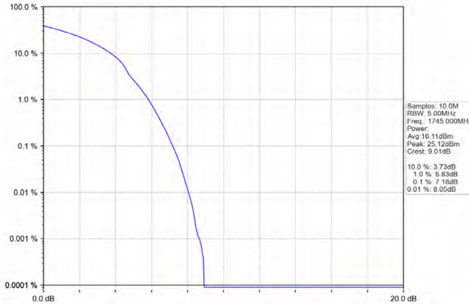
Band 4 20MHz 16QAM HCH 1745MHz RB 100 0 NTV
