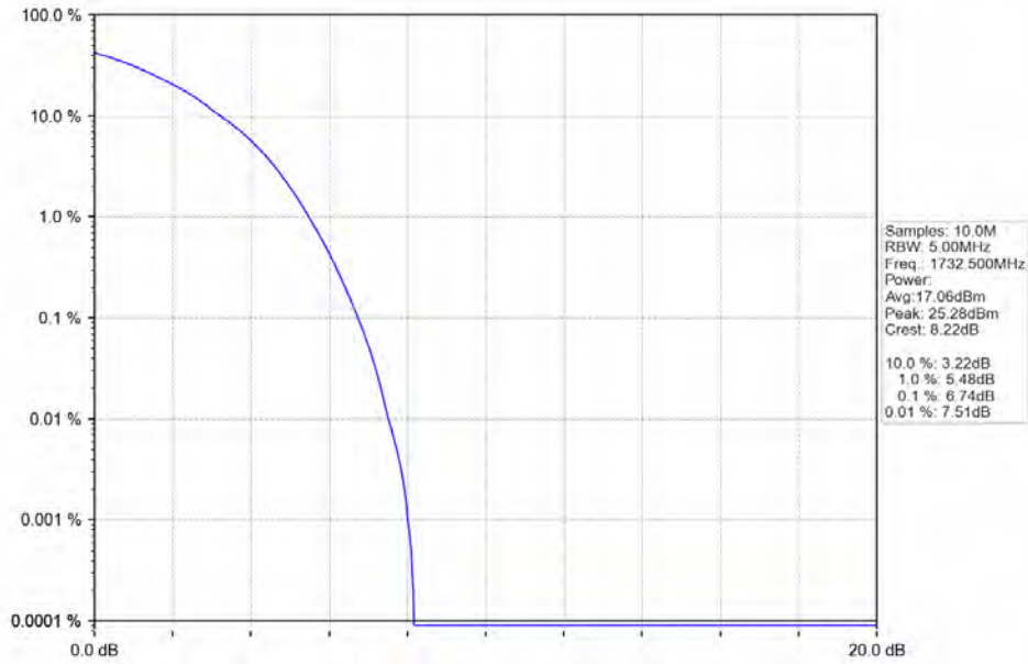
Band 4 15MHz 64QAM MCH 1732.5MHz RB 75 0 NTVN
