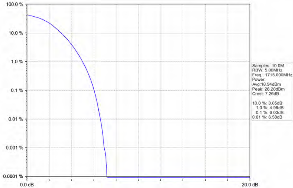
Band 4 10MHz 64QAM LCH 1715MHz RB 50 0 NTVN
