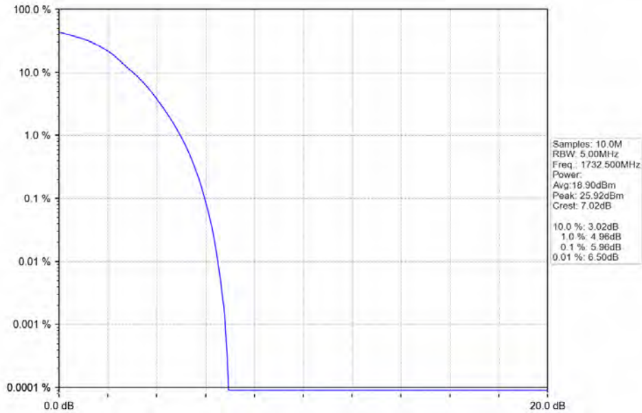
Band 4 10MHz 64QAM MCH 1732.5MHz RB 50 0 NTVN
