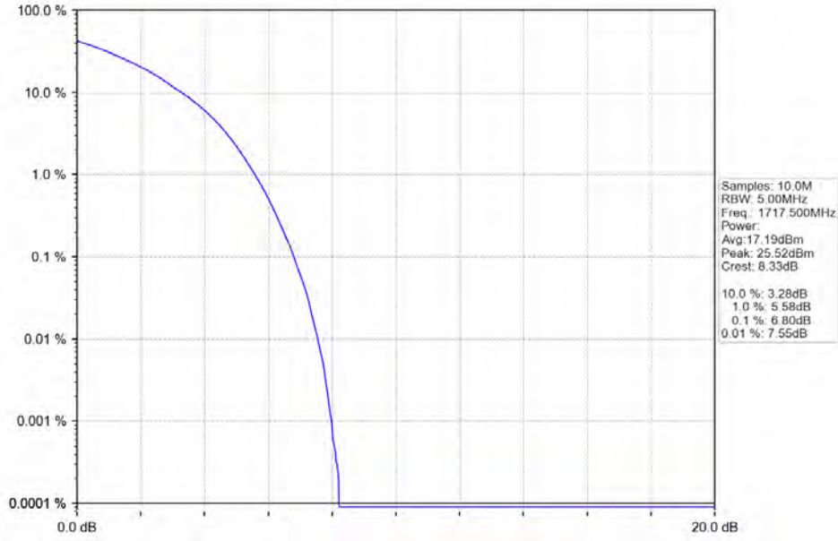
Band 4 15MHz 64QAM LCH 1717.5MHz RB 75 0 NTVN
