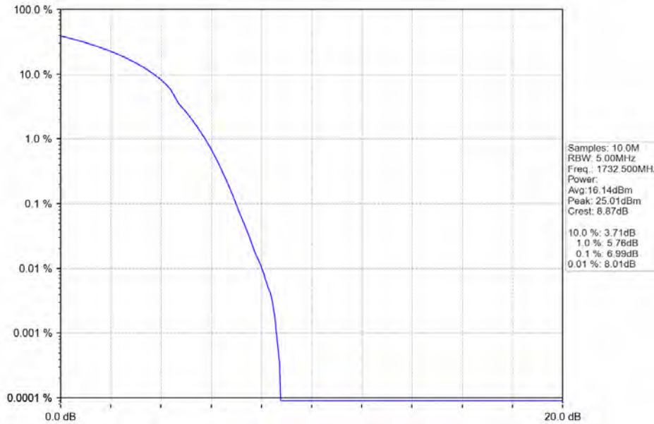
Band 4 20MHz 16QAM MCH 1732.5MHz RB 100 0 NTV
