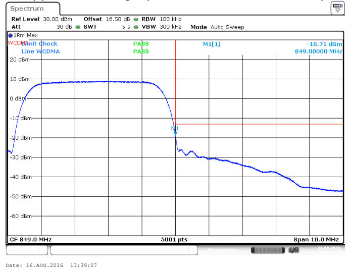
Upper Band Edge (Channel 4233, 846.6 MHz)
