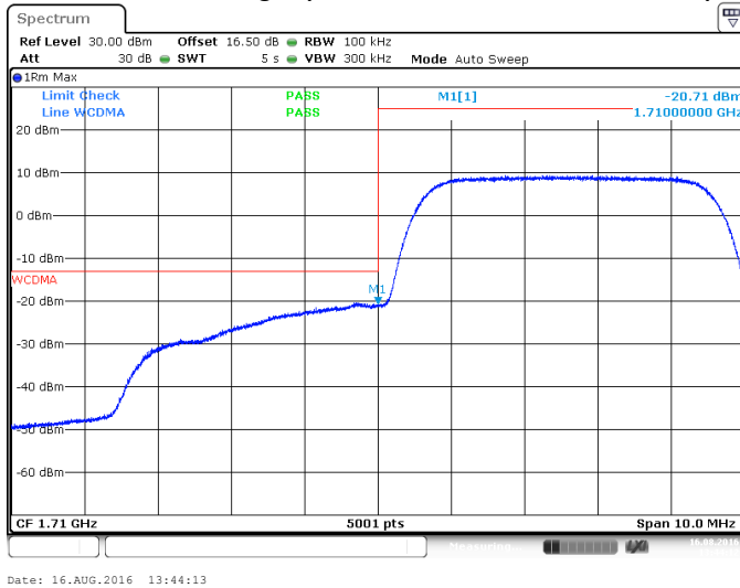
Lower Band Edge (Channel 1313, 1712.6 MHz)
