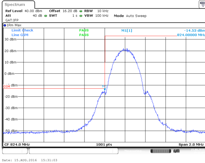
Lower Band Edge (Channel 128, 824.2 MHz)
