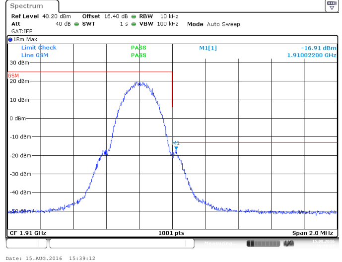
Upper Band Edge (Channel 810, 1909.8 MHz)
