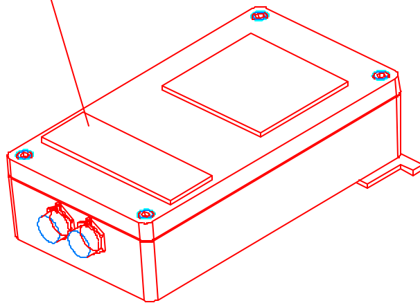
VIP110-24, Isometric View
