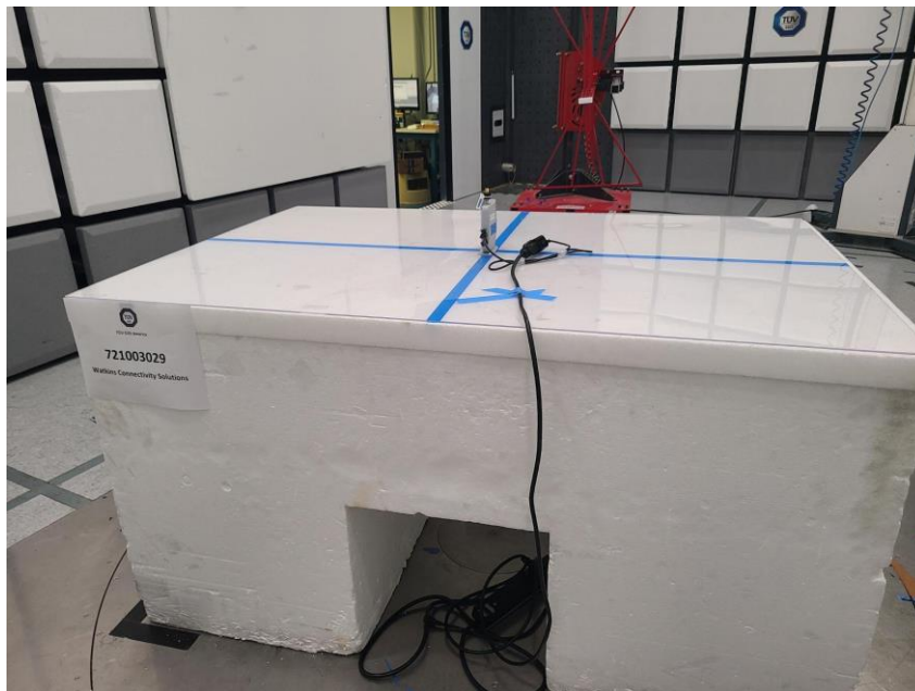
Radiated Emissions Test Setup (30MHz to 1GHz)
