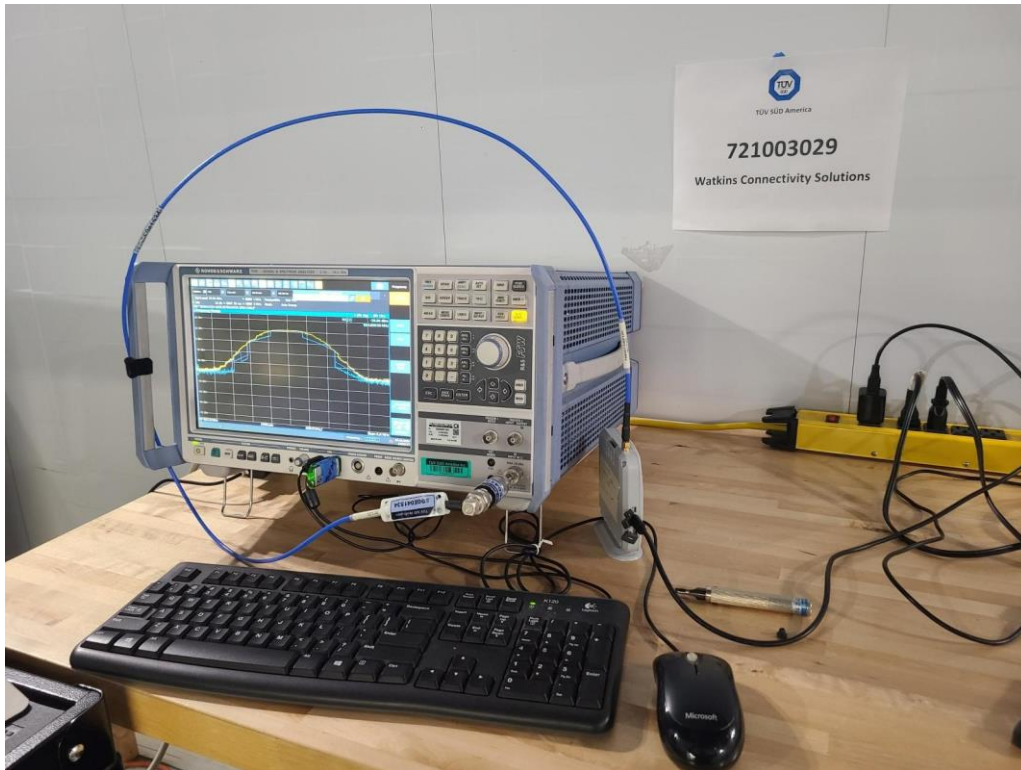
Antenna Conducted Port Test Setup
