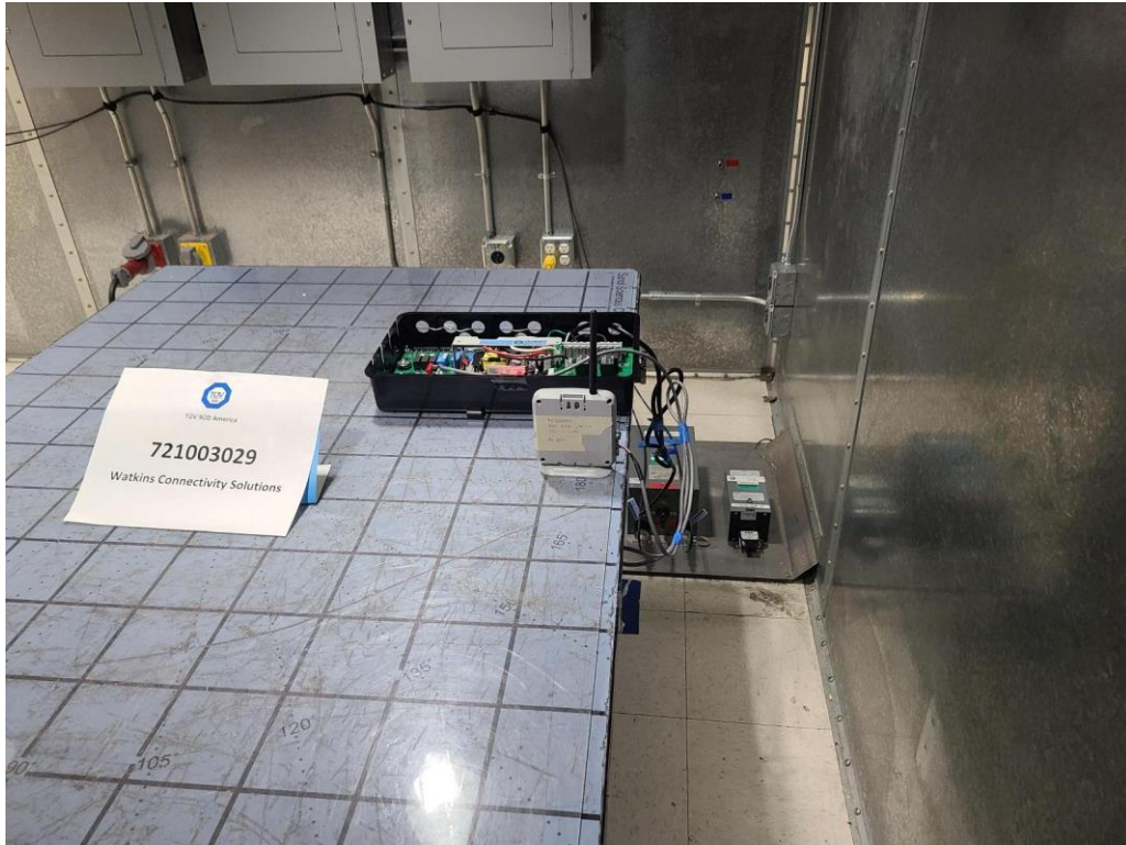
AC Mains Conducted Emissions Test Setup - SNA
