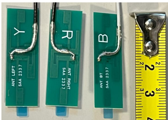
Antennas front side.
