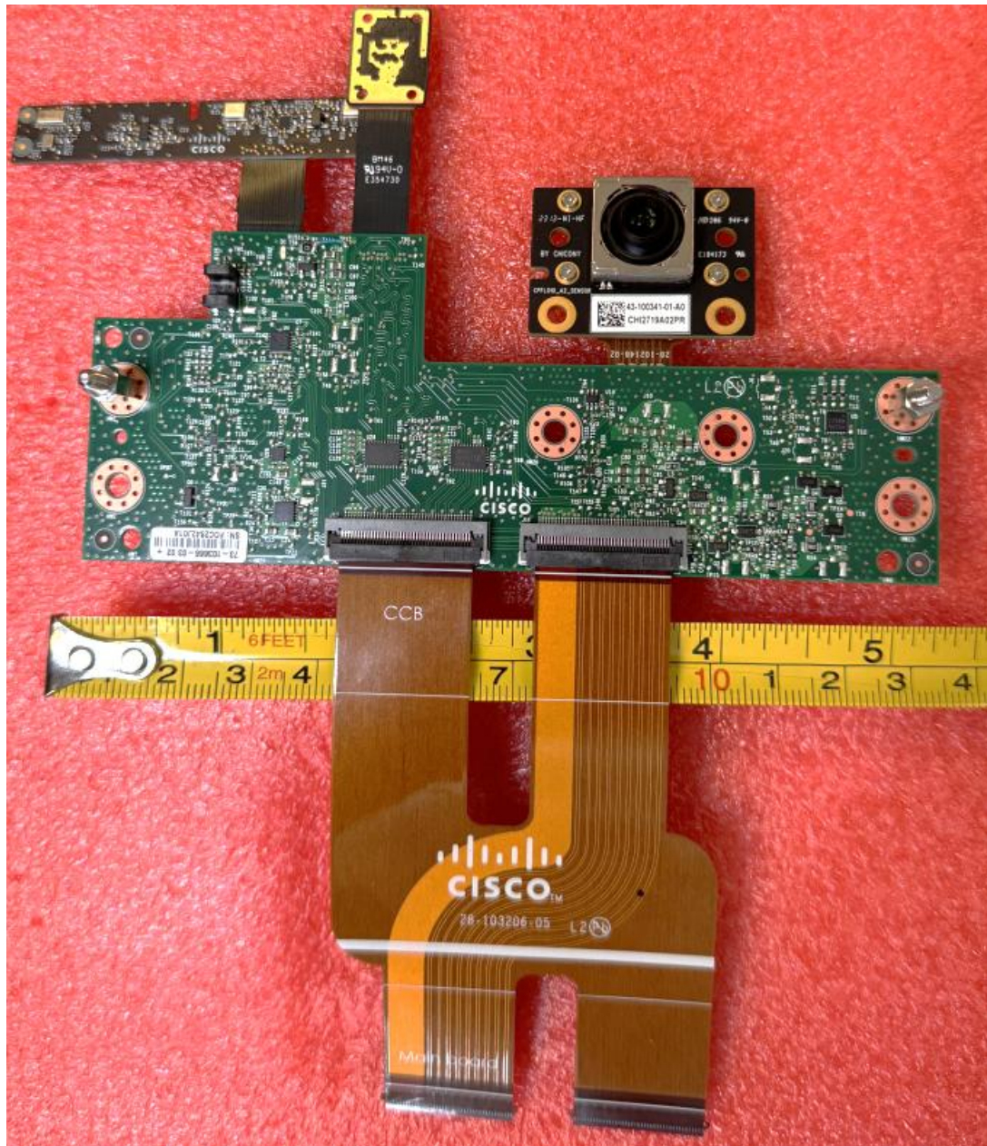
Camera baseboard front side. Cameras and mic board.
