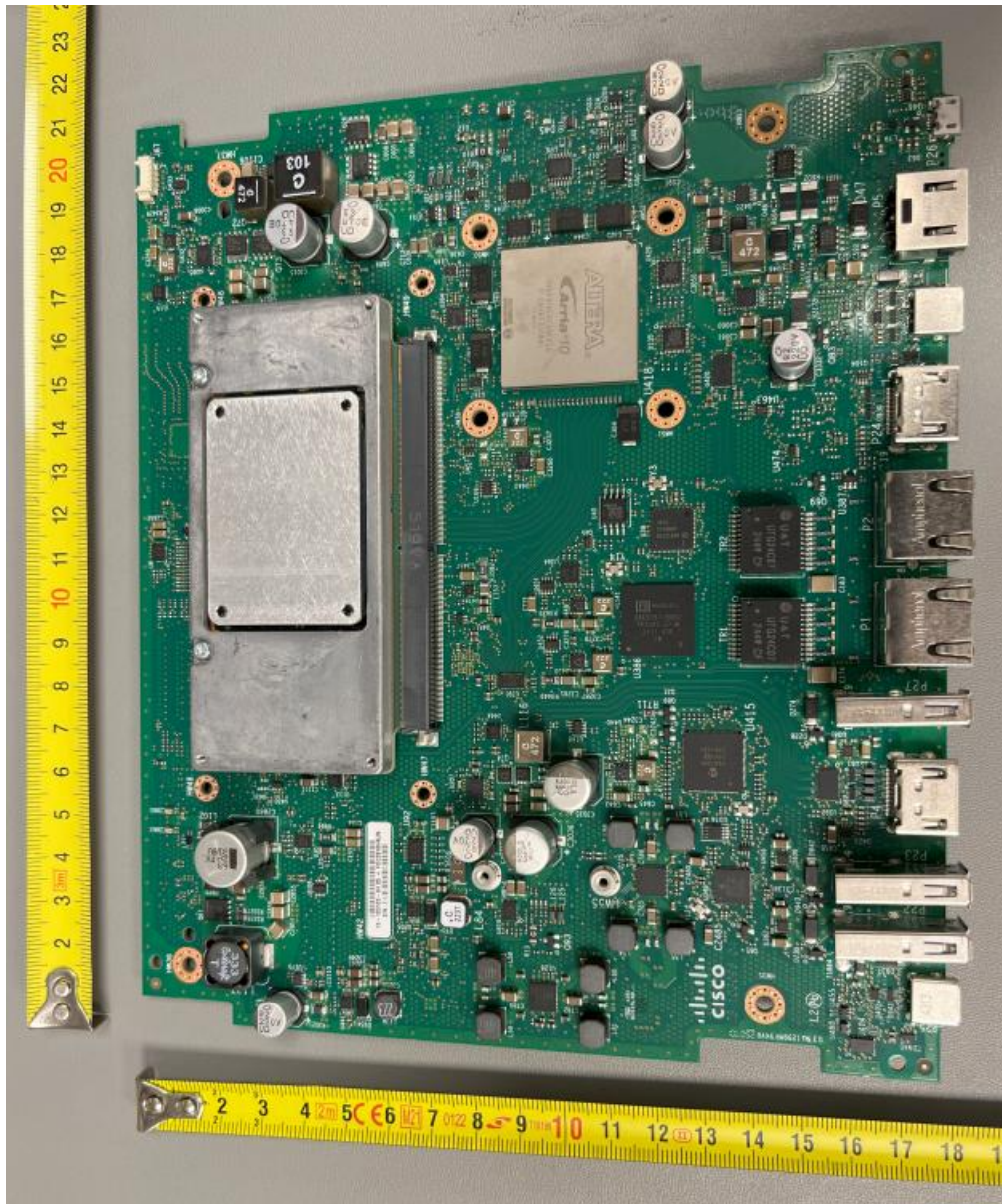
Mainboard top side
