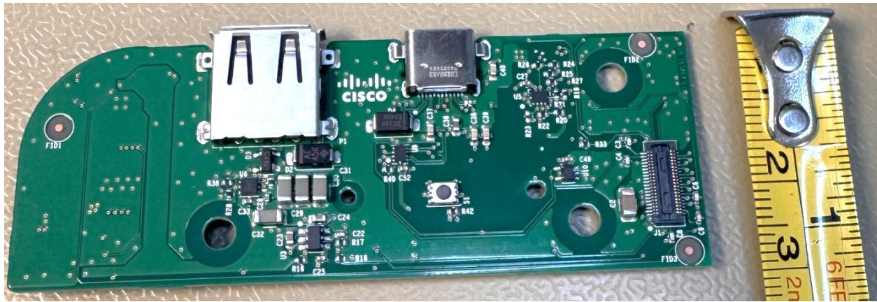
Side IO board top
