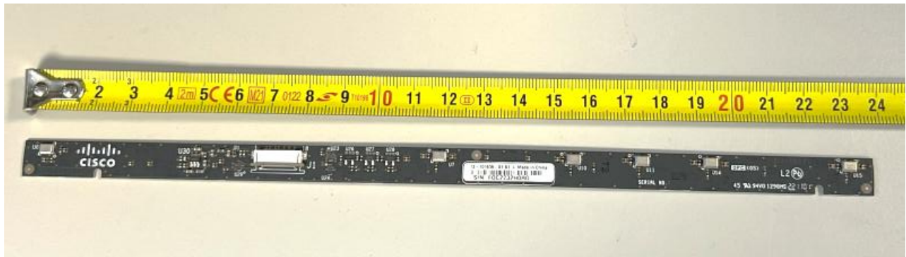
Mic board 6 MEMS front side
