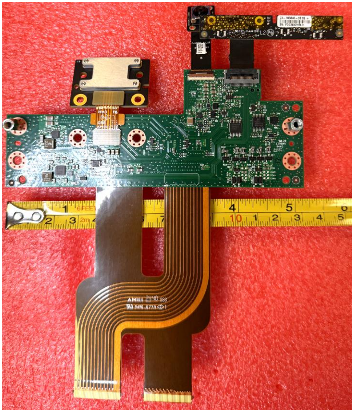
Camera base board rear side. Cameras and mic board.
