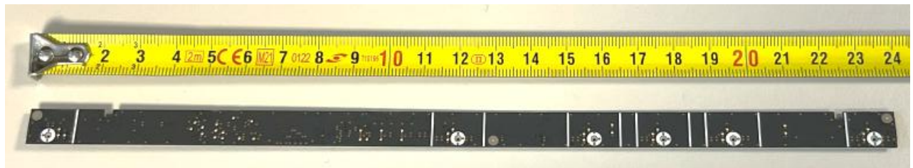
Mic board 6 MEMS rear side
