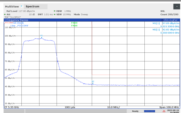
Band Edge, 5350 MHz, Ch064, 802.11n MCS8 MIMO, Av, Max
