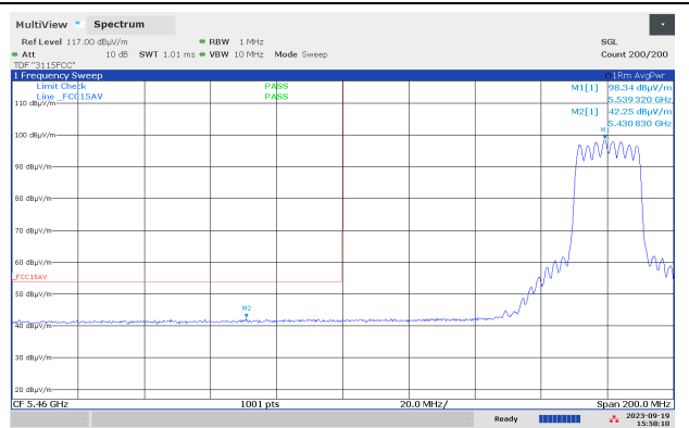
Band Edge, 5460 MHz, Ch108, 802.11ax MCS0 MIMO, Av, Max
