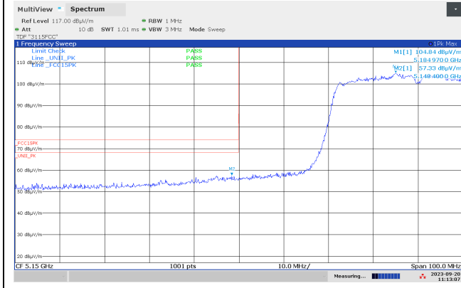
Band Edge 5150 MHz, ch038, 802.11n MCS8 HT40 MIMO, Radiated, Max
