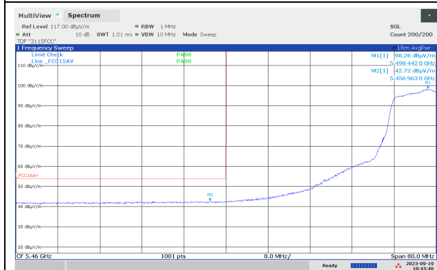
Band Edge, 5460 MHz, Ch100, 802.11a 6M, Av, Max
