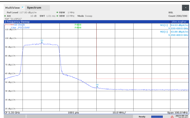
Band Edge, 5350 MHz, Ch064, 802.11ax MCS0 SISO, Av, Max
