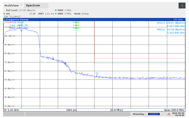
Band Edge 5350 MHz, ch054, 802.11n MCS0 HT40, Radiated, Max
