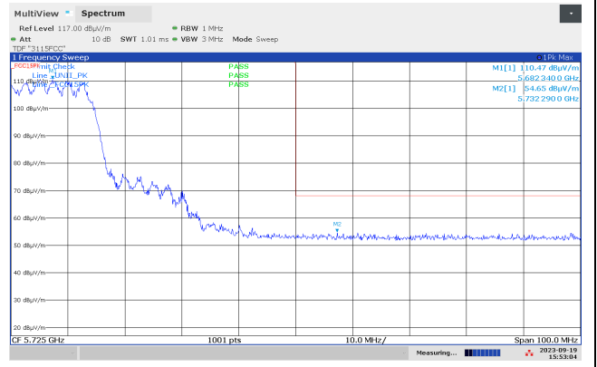
Band Edge 5725 MHz, ch136, 802.11ax MCS0 MIMO, Radiated, Max
