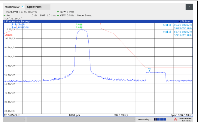
Band Edge 5850 MHz, ch157, 802.11a 6Mb, Radiated, Max
