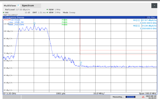
Band Edge 5350 MHz, ch064, 802.11ax MCS0 MIMO, Radiated, Max
