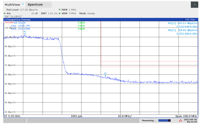
Band Edge 5350 MHz, ch062, 802.11ax MCS0 HT40 SISO, Radiated, Max
