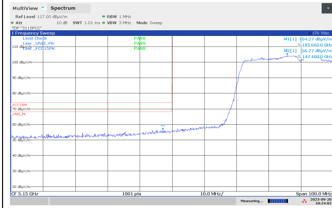
Band Edge 5150 MHz, ch038, 802.11n MCS0 HT40, Radiated, Max
