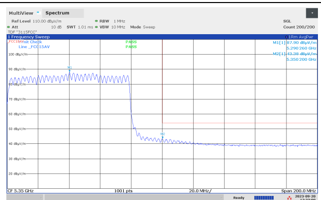
Band Edge, 5350 MHz, Ch058, 802.11ax MCS0 HT80 MIMO, Av, Max
