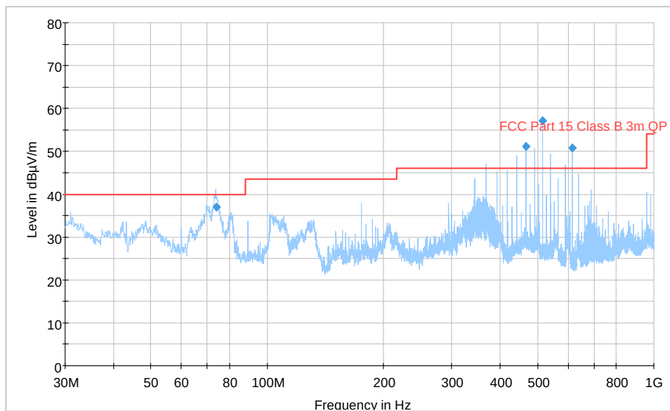
Radiated Emissions, 30-1000 MHz
