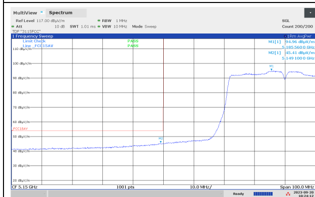
Band Edge, 5150 MHz, Ch038, 802.11n MCS0 HT40 SISO, Av, Max
