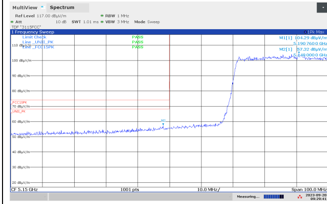
Band Edge 5150 MHz, ch038, 802.11ax MCS0 HT40 SISO, Radiated, Max
