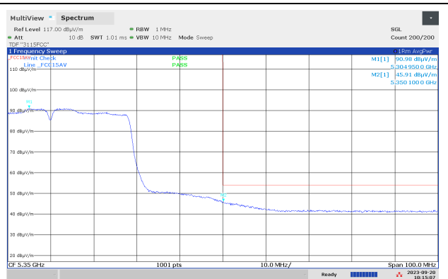
Band Edge, 5350 MHz, Ch062, 802.11n MCS0 HT40 SISO, Av, Max
