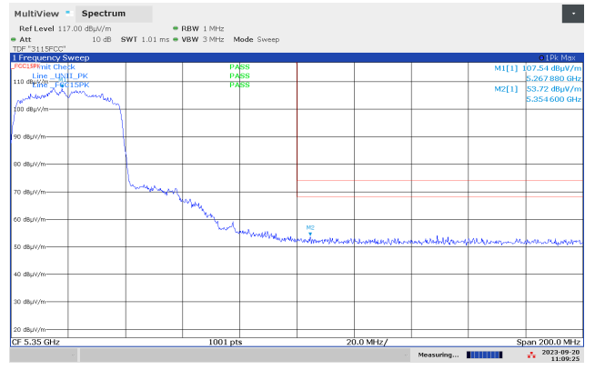
Band Edge 5350 MHz, ch054, 802.11n MCS8 HT40 MIMO, Radiated, Max
