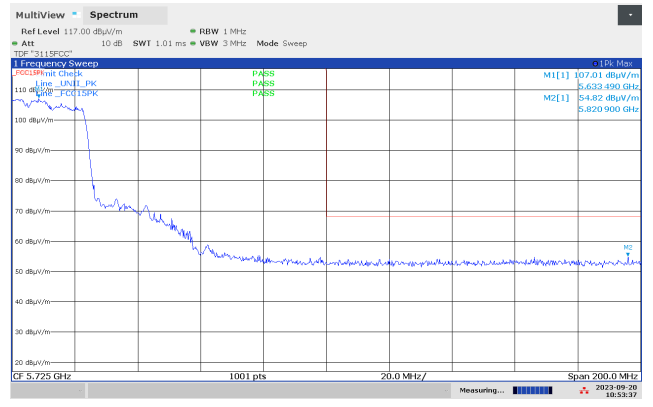
Band Edge 5725 MHz, ch126, 802.11n MCS8 HT40 MIMO, Radiated, Max
