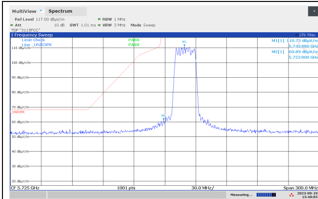
Band Edge 5725 MHz, ch149, 802.11ax MCS0 MIMO, Radiated, Max
