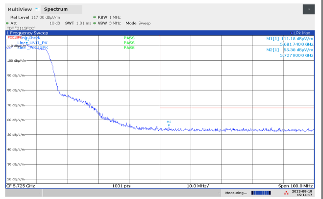
Band Edge 5725 MHz, ch136, 802.11n MCS8 MIMO, Radiated, Max
