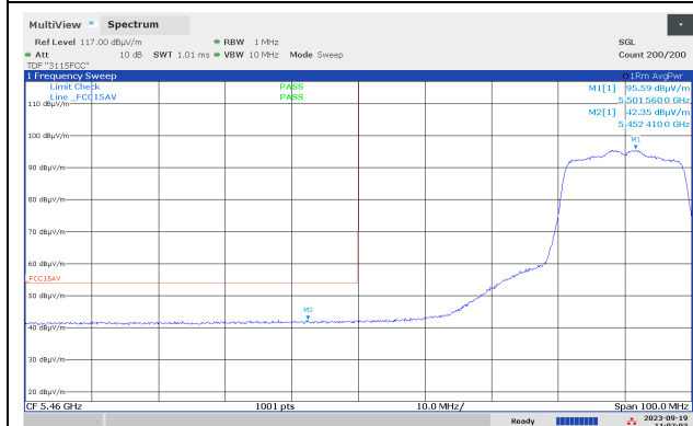
Band Edge, 5460 MHz, Ch100, 802.11n MCS0, Av, Max
