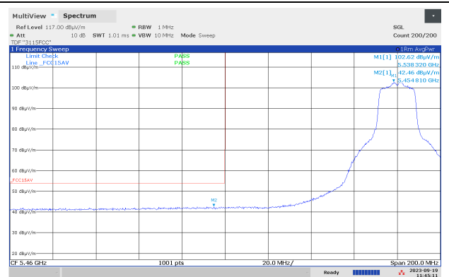
Band Edge, 5460 MHz, Ch108, 802.11a 6M, Av, Max
