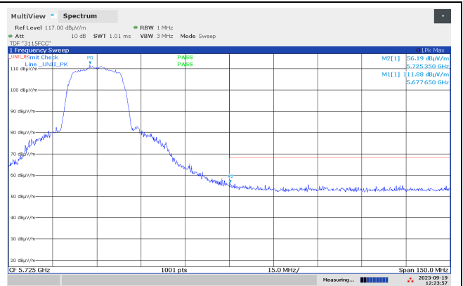
Band Edge 5725 MHz, ch136, 802.11n MCS0, Radiated, Max
