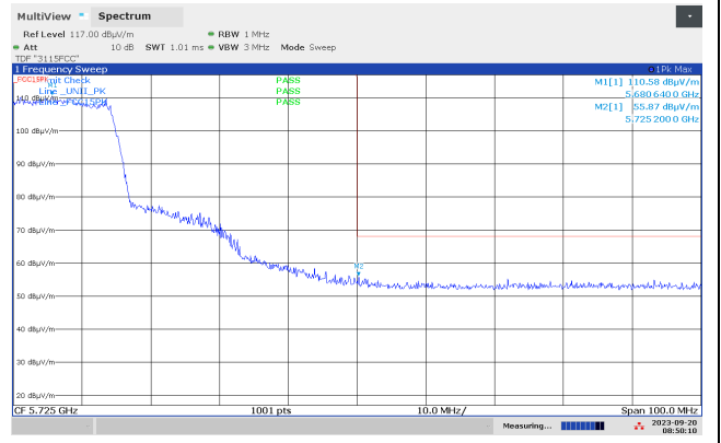
Band Edge 5725 MHz, ch136, 802.11ax MCS0 SISO, Radiated, Max
