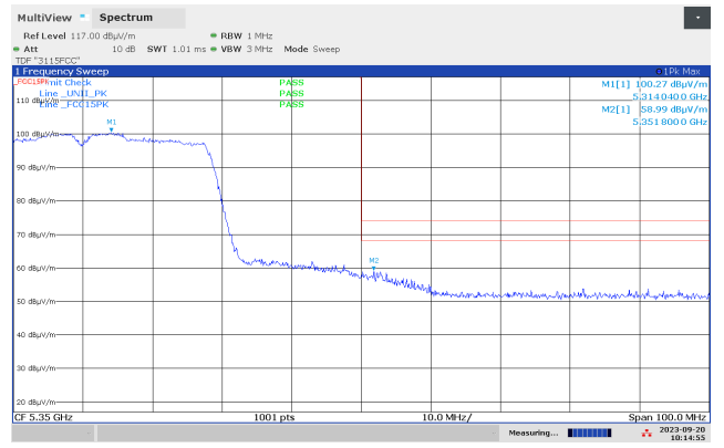
Band Edge 5350 MHz, ch062, 802.11n MCS0 HT40, Radiated, Max
