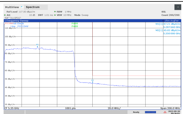
Band Edge, 5350 MHz, Ch058, 802.11ax MCS0 HT80 SISO, Av, Max
