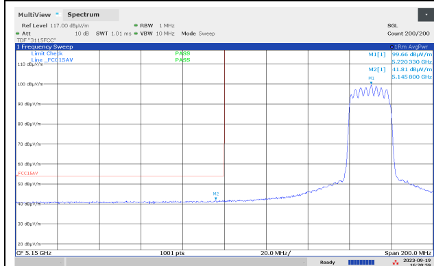
Band Edge, 5150 MHz, Ch044, 802.11ax MCS0 MIMO, Av, Max
