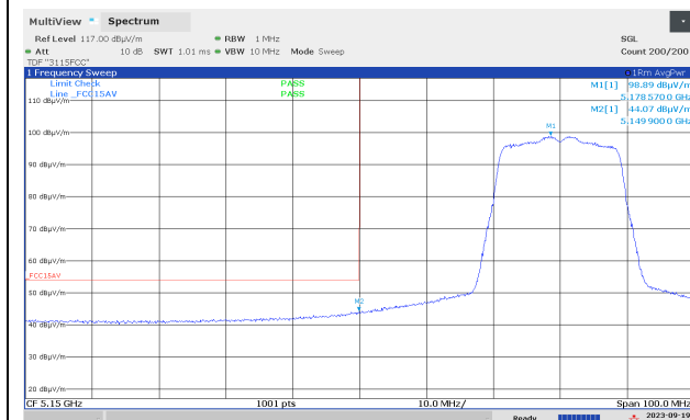
Band Edge, 5150 MHz, Ch036, 802.11n MCS0, Av, Max
