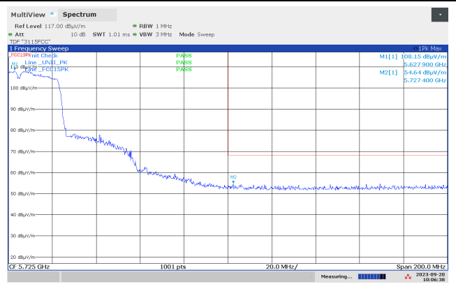
Band Edge 5725 MHz, ch126, 802.11n MCS0 HT40, Radiated, Max
