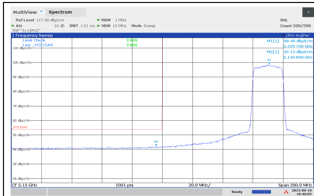
Band Edge, 5150 MHz, Ch044, 802.11ax MCS0 SISO, Av, Max
