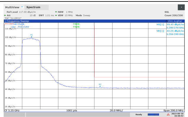
Band Edge, 5350 MHz, Ch056, 802.11ax MCS0 SISO, Av, Max
