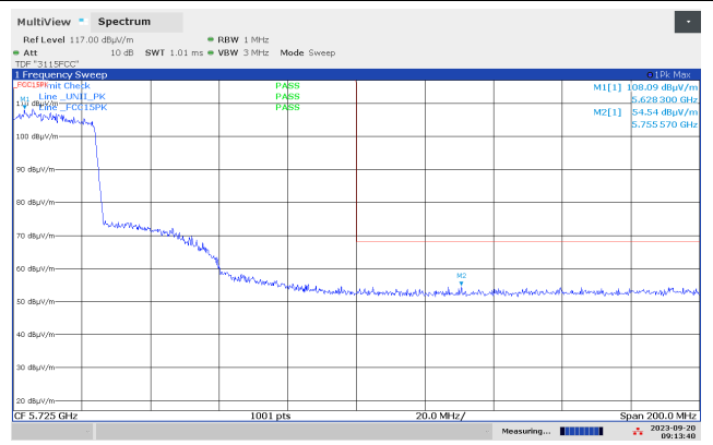
Band Edge 5725 MHz, ch126, 802.11ax MCS0 HT40, Radiated, Max
