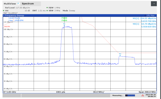
Band Edge 5850 MHz, ch165, 802.11ax MCS0 SISO, Radiated, Max
