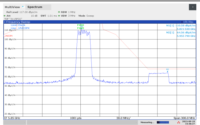
Band Edge 5850 MHz, ch165, 802.11ax MCS0 MIMO, Radiated, Max
