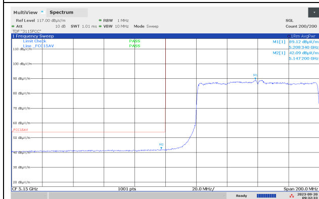
Band Edge, 5150 MHz, Ch042, 802.11ax MCS0 HT80 SISO, Av, Max
