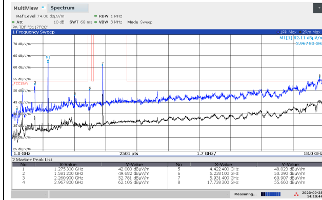
Radiated Emissions 1-18 GHz, Ch048, 802.11n MCS8, MIMO, HP
