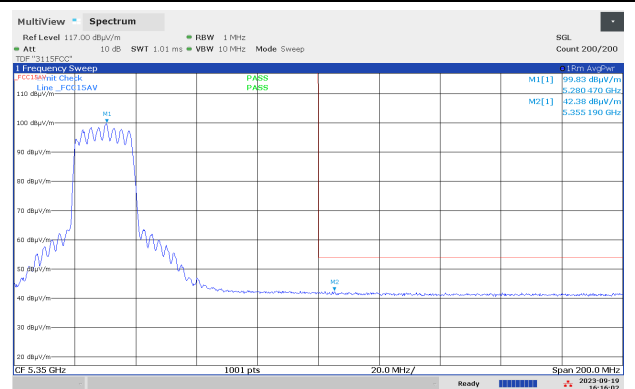
Band Edge, 5350 MHz, Ch056, 802.11ax MCS0 MIMO, Av, Max
