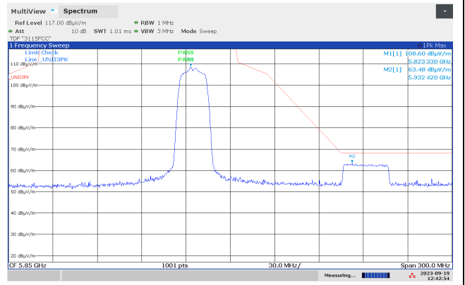
Band Edge 5850 MHz, ch157, 802.11n MCS0, Radiated, Max
