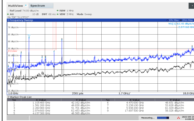
Radiated Emissions 1-18 GHz, Ch048, 802.11n MCS0, Ant 1, HP
