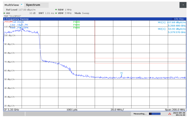
Band Edge 5350 MHz, ch054, 802.11ax MCS0 HT40 SISO, Radiated, Max
