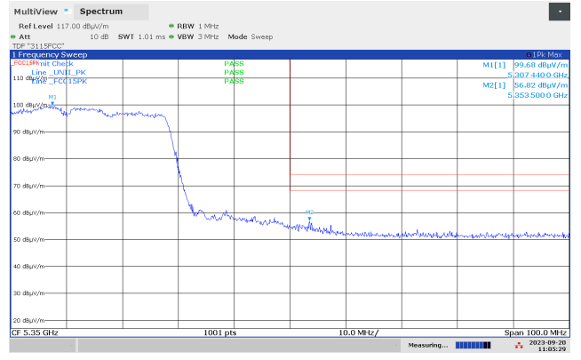
Band Edge 5350 MHz, ch062, 802.11n MCS8 MIMO, Radiated, Max
