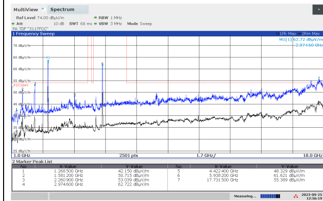
Radiated Emissions 1-18 GHz, Ch116, 802.11ax MCS0, Ant 1, HP
