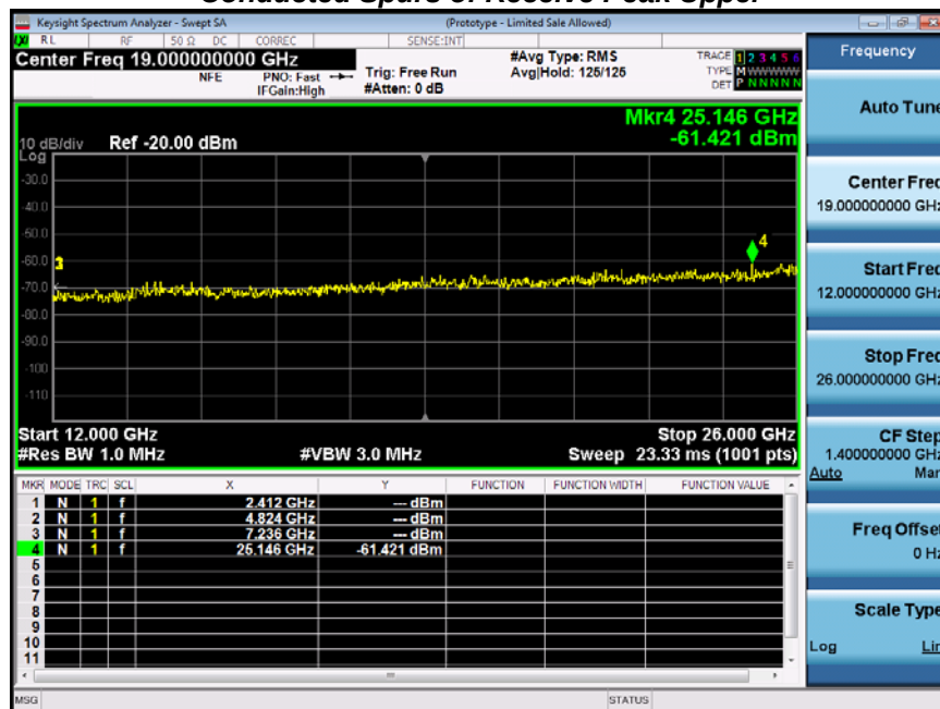
Conducted Spurs of Receive Peak Upper
