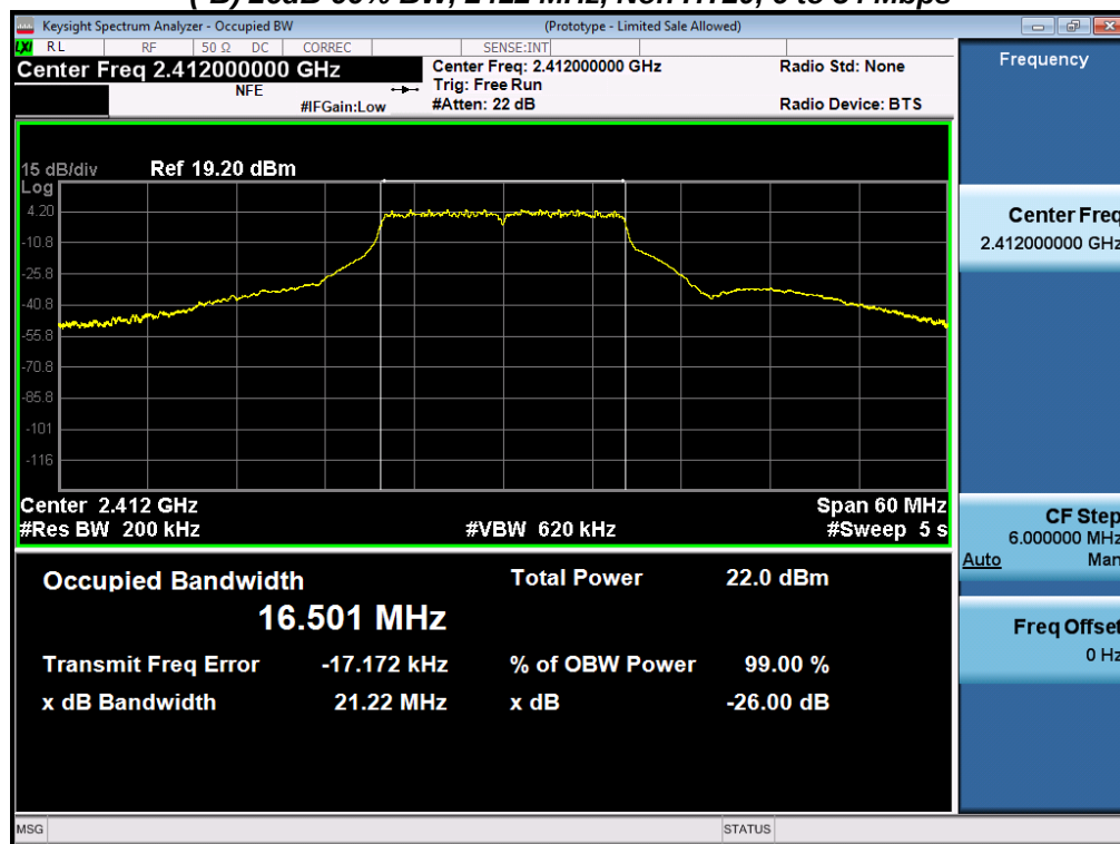
(-B) 26dB-99% BW, 2412 MHz, Non HT20, 6 to 54 Mbps
