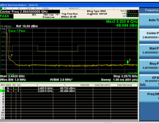
Antenna D
