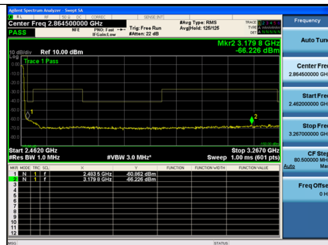
Antenna D
