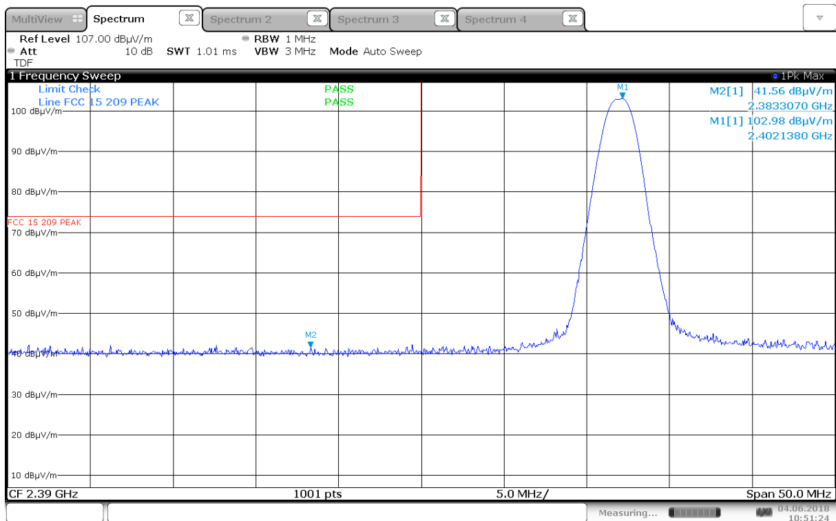
Lower Band Edge, 2402MHz, 8PSK, Peak, (Max: HP)
