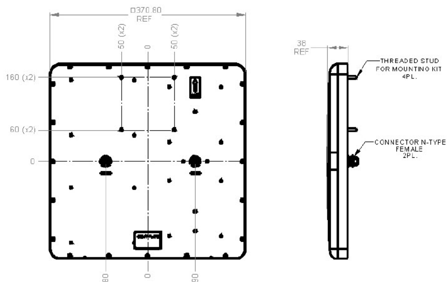
Figure 2: Mechanical Drawing
