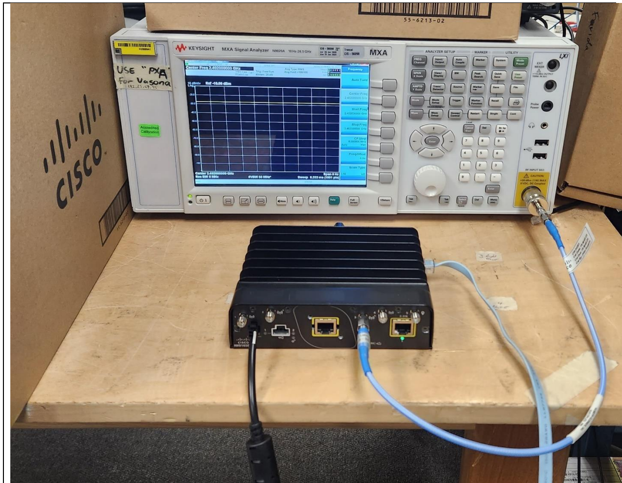
Title: BLE Conducted Test Configuration
