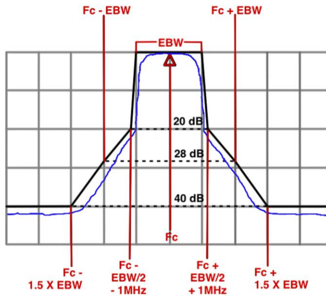
Figure 5. Generic Emission Mask
