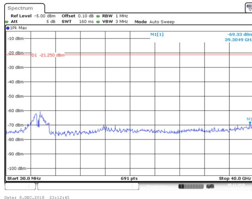
Ant-b
