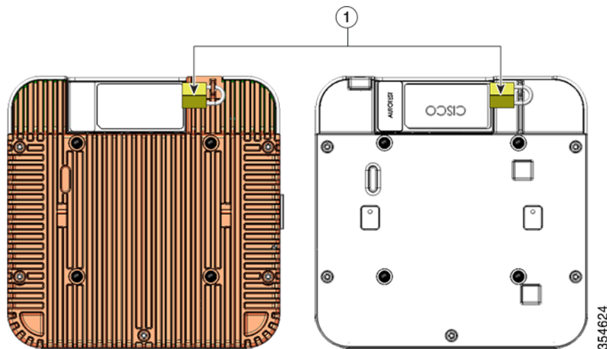
Figure 4 Locking the AP to the Bracket
