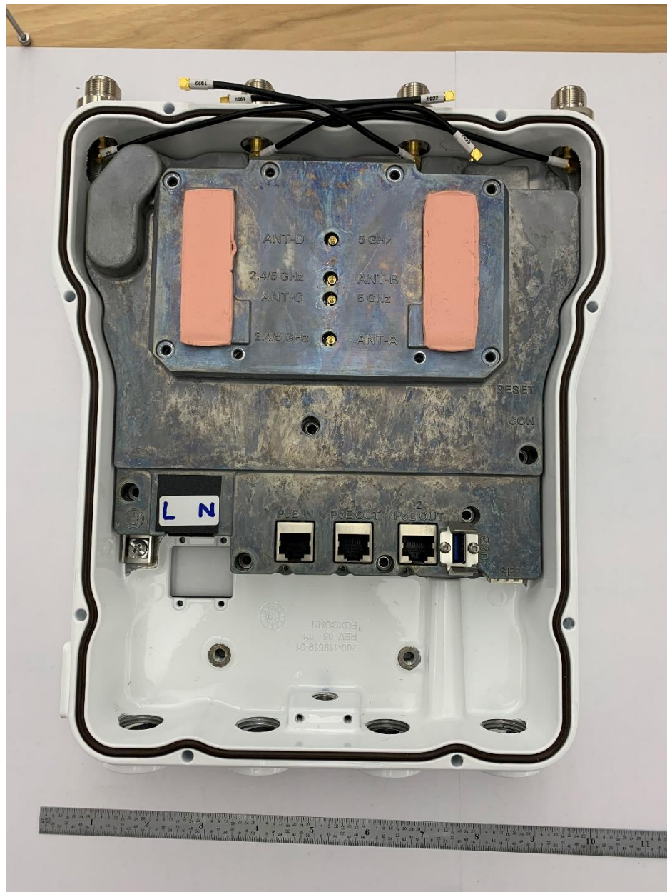
Closer view of the LDKESW6300 module in the product
