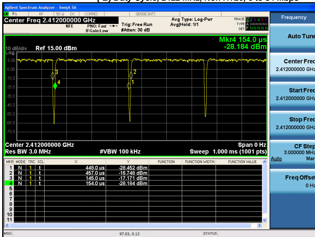
(-B) Duty Cycle, 2412 MHz, Non HT20, 6 to 54 Mbps
