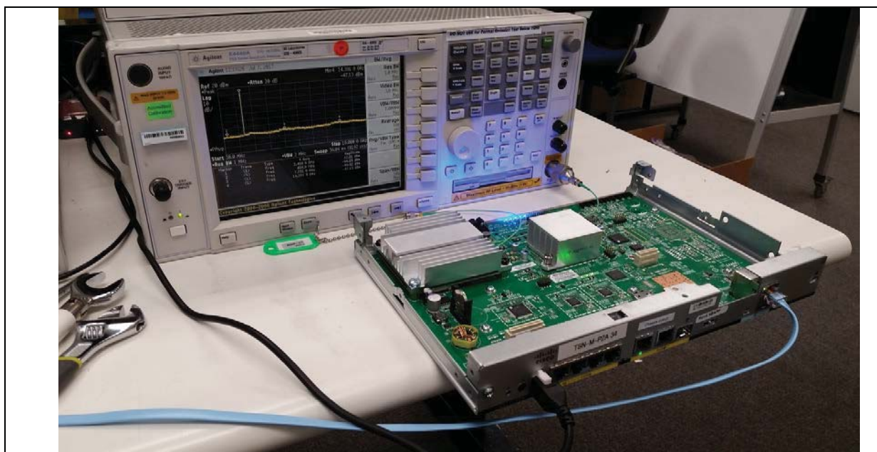
Title: Conducted Setup (Conducted Spurious Emissions)
