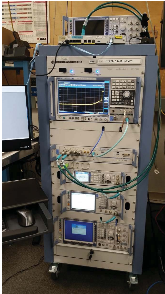
Title: Conducted Setup (Band Edge)
