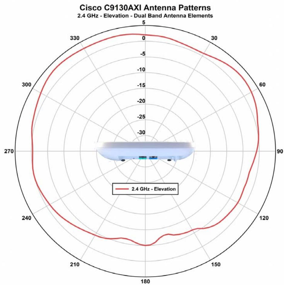
Figure 3-6 C9130AXI - Dual-band Antenna radiation pattern (2.4 GHz Elevation)
