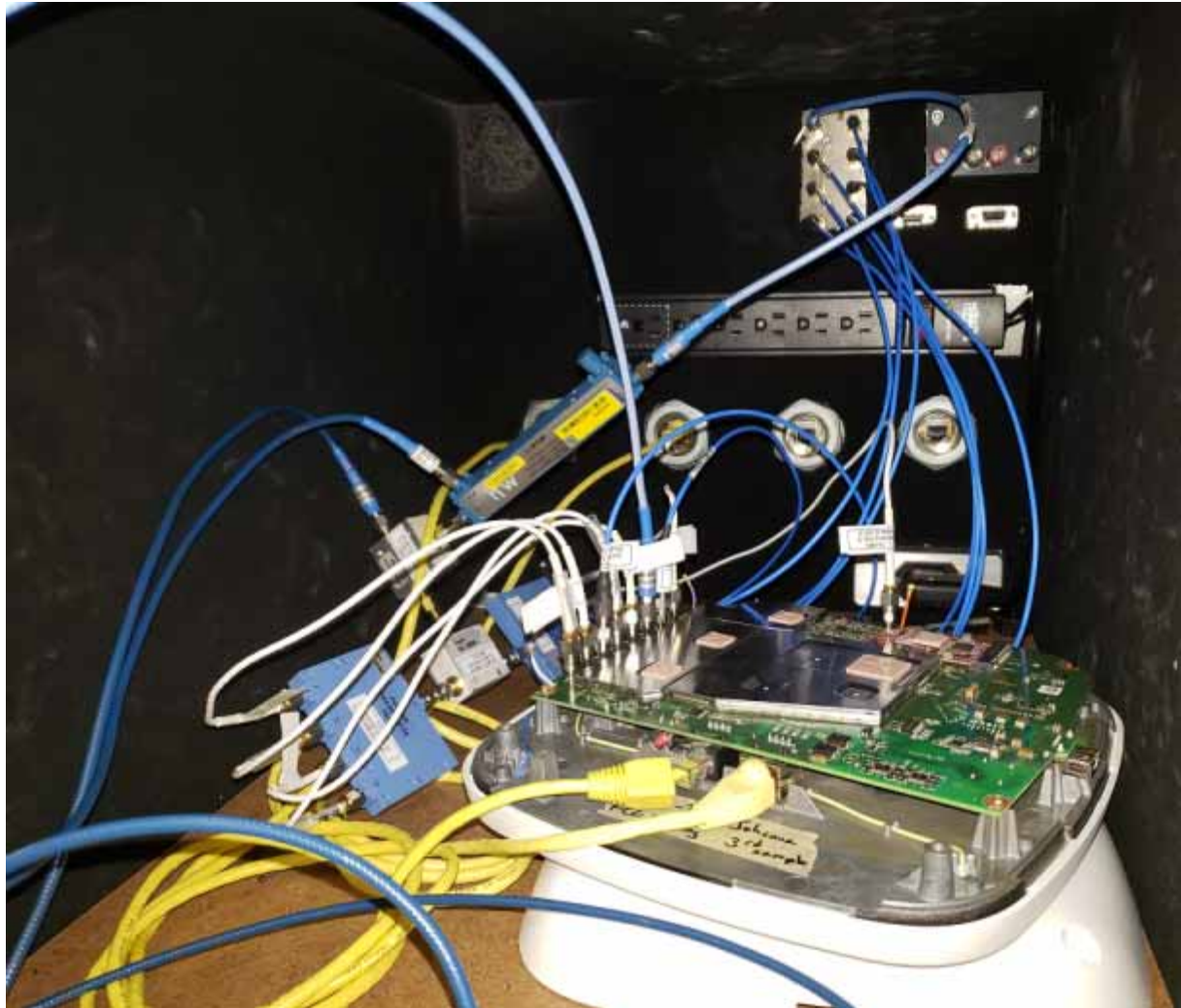
Title: Radio Conducted DFS Test Setup
