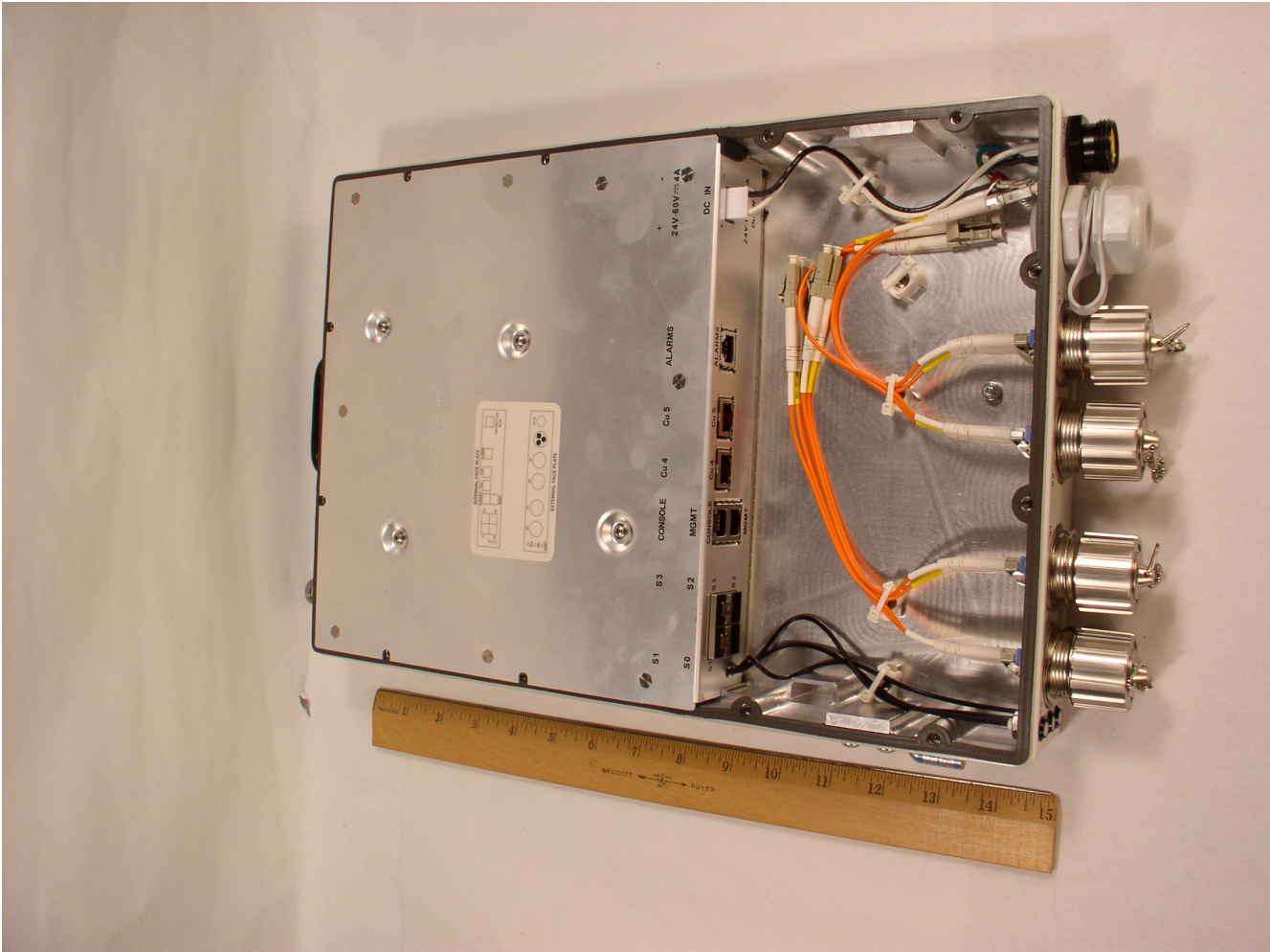
ASR901S router with Lid removed
