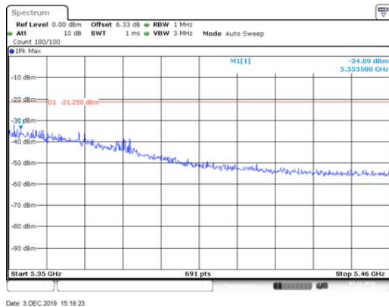
HE80, M0.1 to M11.1 5290 MHz Peak
