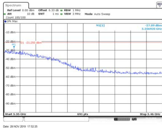
VHT80, M0.1 to M9.1 5290 MHz Peak
