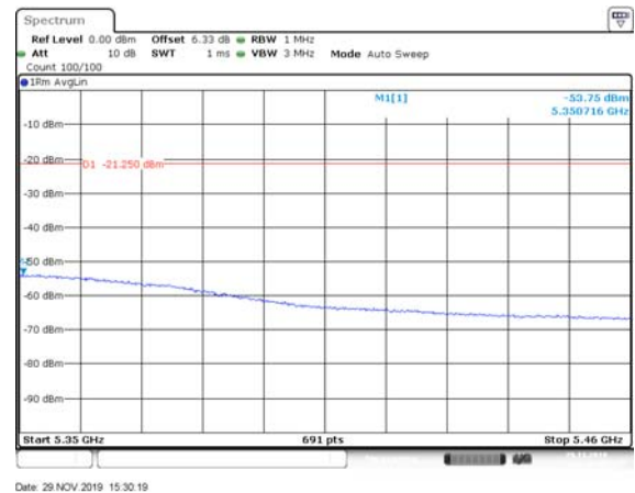
VHT80, M0.1 to M9.1 5290 MHz Average
