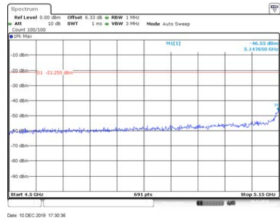
HT/VHT40, M0 to M7, M0.1 to M9.1 5190 MHz Average
