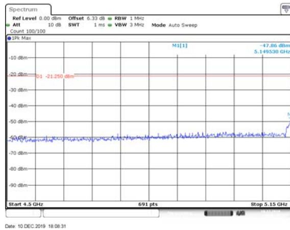
HT/VHT40, M0 to M7, M0.1 to M9.1-BF 5190 MHz Peak
