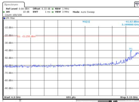
VHT80, M0.1 to M9.1 5210 MHz Peak
